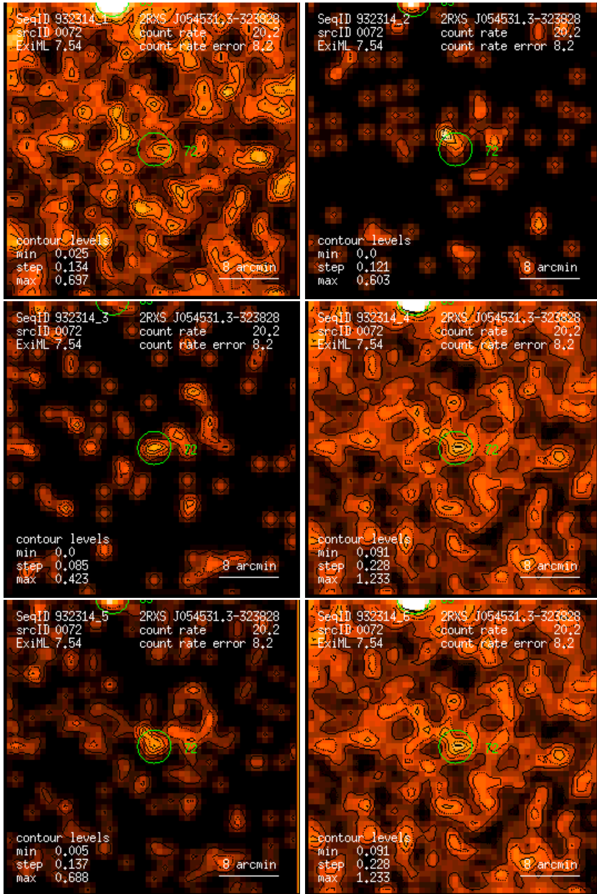
Figure 72: RASS 932314: detection 0072: band rate images, Gaussian filter: (1) PSPC channels 11 – 41, (2) 52 – 90, (3) 91 – 201, (4) 11 – 235, (5) 52 – 201, (6) 11 – 201. Broad band rates in counts/ks. Band rate contour levels in counts/ks/arcmin 2 .
