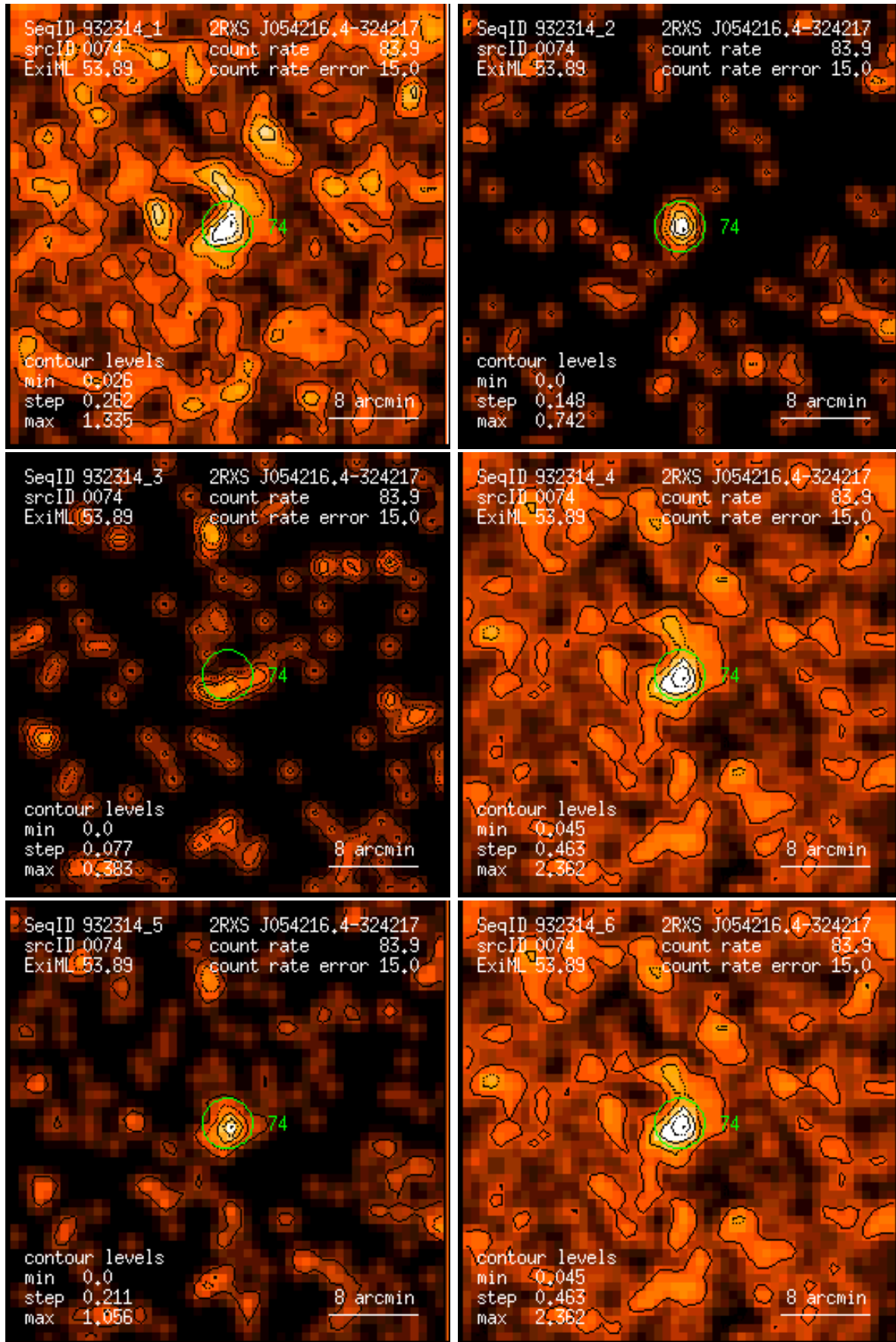
Figure 74: RASS 932314: detection 0074: band rate images, Gaussian filter: (1) PSPC channels 11 – 41, (2) 52 – 90, (3) 91 – 201, (4) 11 – 235, (5) 52 – 201, (6) 11 – 201. Broad band rates in counts/ks. Band rate contour levels in counts/ks/arcmin 2 .
