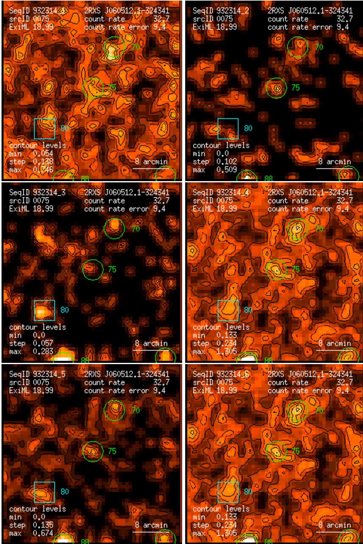
Figure 75: RASS 932314: detection 0075: band rate images, Gaussian filter: (1) PSPC channels 11 – 41, (2) 52 – 90, (3) 91 – 201, (4) 11 – 235, (5) 52 – 201, (6) 11 – 201. Broad band rates in counts/ks. Band rate contour levels in counts/ks/arcmin 2 .
