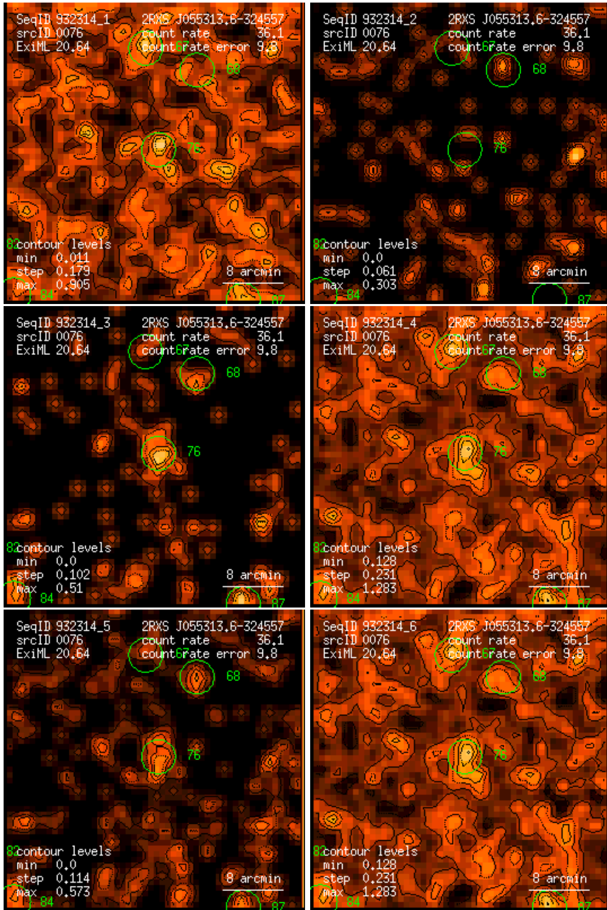
Figure 76: RASS 932314: detection 0076: band rate images, Gaussian filter: (1) PSPC channels 11 – 41, (2) 52 – 90, (3) 91 – 201, (4) 11 – 235, (5) 52 – 201, (6) 11 – 201. Broad band rates in counts/ks. Band rate contour levels in counts/ks/arcmin 2 .
