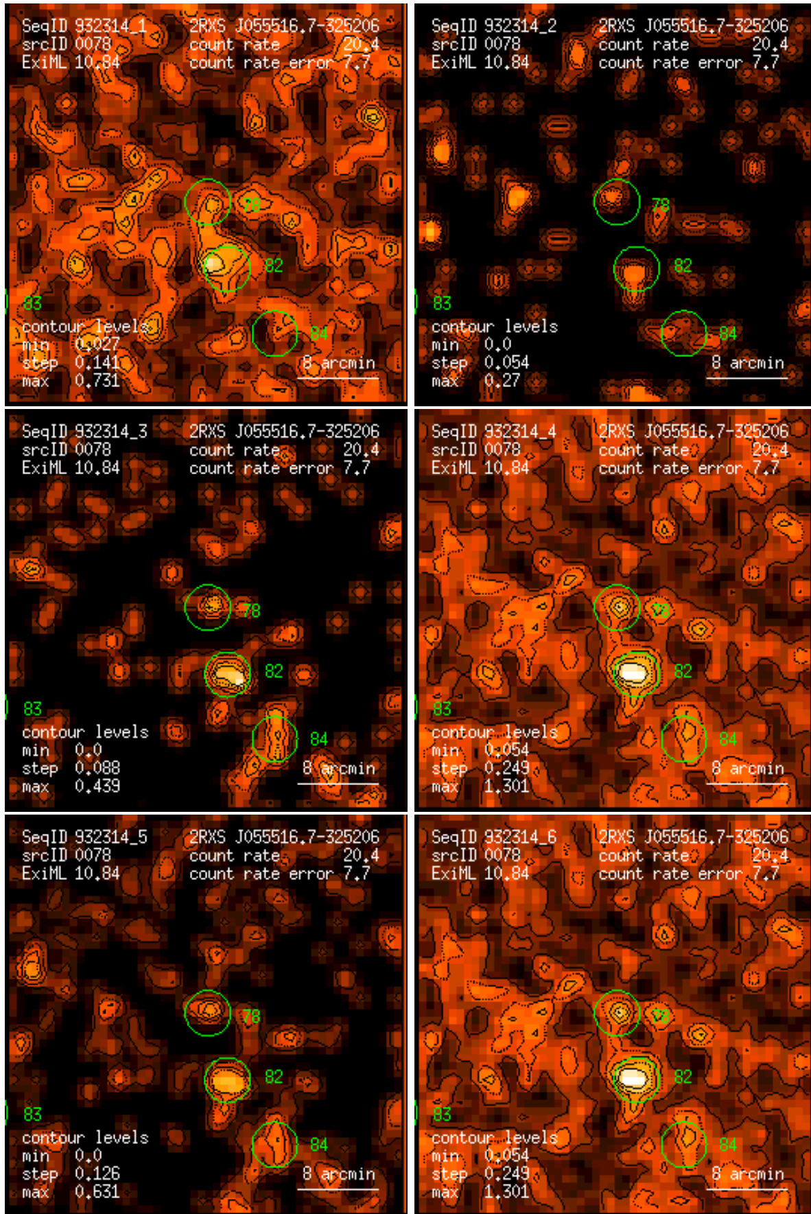
Figure 78: RASS 932314: detection 0078: band rate images, Gaussian filter: (1) PSPC channels 11 – 41, (2) 52 – 90, (3) 91 – 201, (4) 11 – 235, (5) 52 – 201, (6) 11 – 201. Broad band rates in counts/ks. Band rate contour levels in counts/ks/arcmin 2 .
