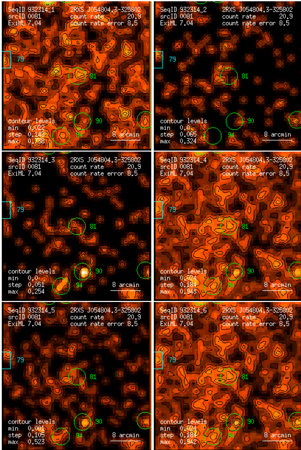
Figure 81: RASS 932314: detection 0081: band rate images, Gaussian filter: (1) PSPC channels 11 – 41, (2) 52 – 90, (3) 91 – 201, (4) 11 – 235, (5) 52 – 201, (6) 11 – 201. Broad band rates in counts/ks. Band rate contour levels in counts/ks/arcmin 2 .
