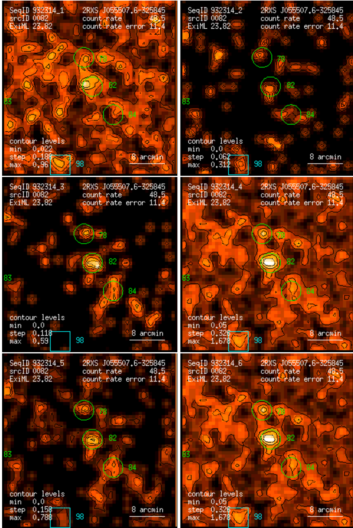
Figure 82: RASS 932314: detection 0082: band rate images, Gaussian filter: (1) PSPC channels 11 – 41, (2) 52 – 90, (3) 91 – 201, (4) 11 – 235, (5) 52 – 201, (6) 11 – 201. Broad band rates in counts/ks. Band rate contour levels in counts/ks/arcmin 2 .
