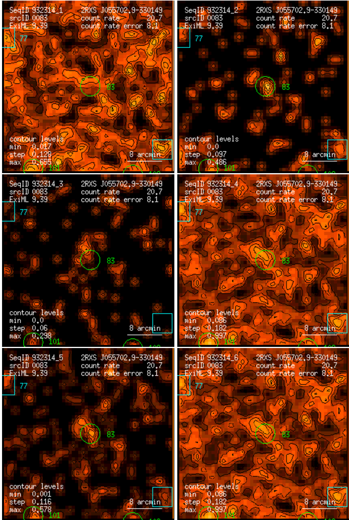
Figure 83: RASS 932314: detection 0083: band rate images, Gaussian filter: (1) PSPC channels 11 – 41, (2) 52 – 90, (3) 91 – 201, (4) 11 – 235, (5) 52 – 201, (6) 11 – 201. Broad band rates in counts/ks. Band rate contour levels in counts/ks/arcmin 2 .
