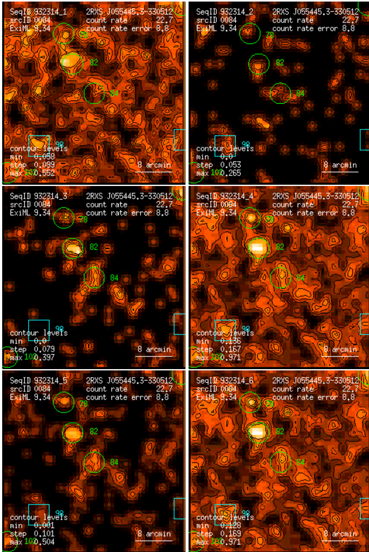
Figure 84: RASS 932314: detection 0084: band rate images, Gaussian filter: (1) PSPC channels 11 – 41, (2) 52 – 90, (3) 91 – 201, (4) 11 – 235, (5) 52 – 201, (6) 11 – 201. Broad band rates in counts/ks. Band rate contour levels in counts/ks/arcmin 2 .
