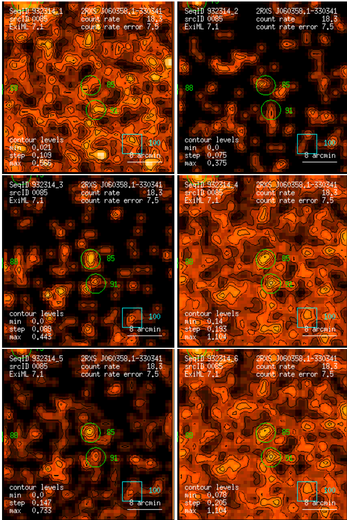
Figure 85: RASS 932314: detection 0085: band rate images, Gaussian filter: (1) PSPC channels 11 – 41, (2) 52 – 90, (3) 91 – 201, (4) 11 – 235, (5) 52 – 201, (6) 11 – 201. Broad band rates in counts/ks. Band rate contour levels in counts/ks/arcmin 2 .
