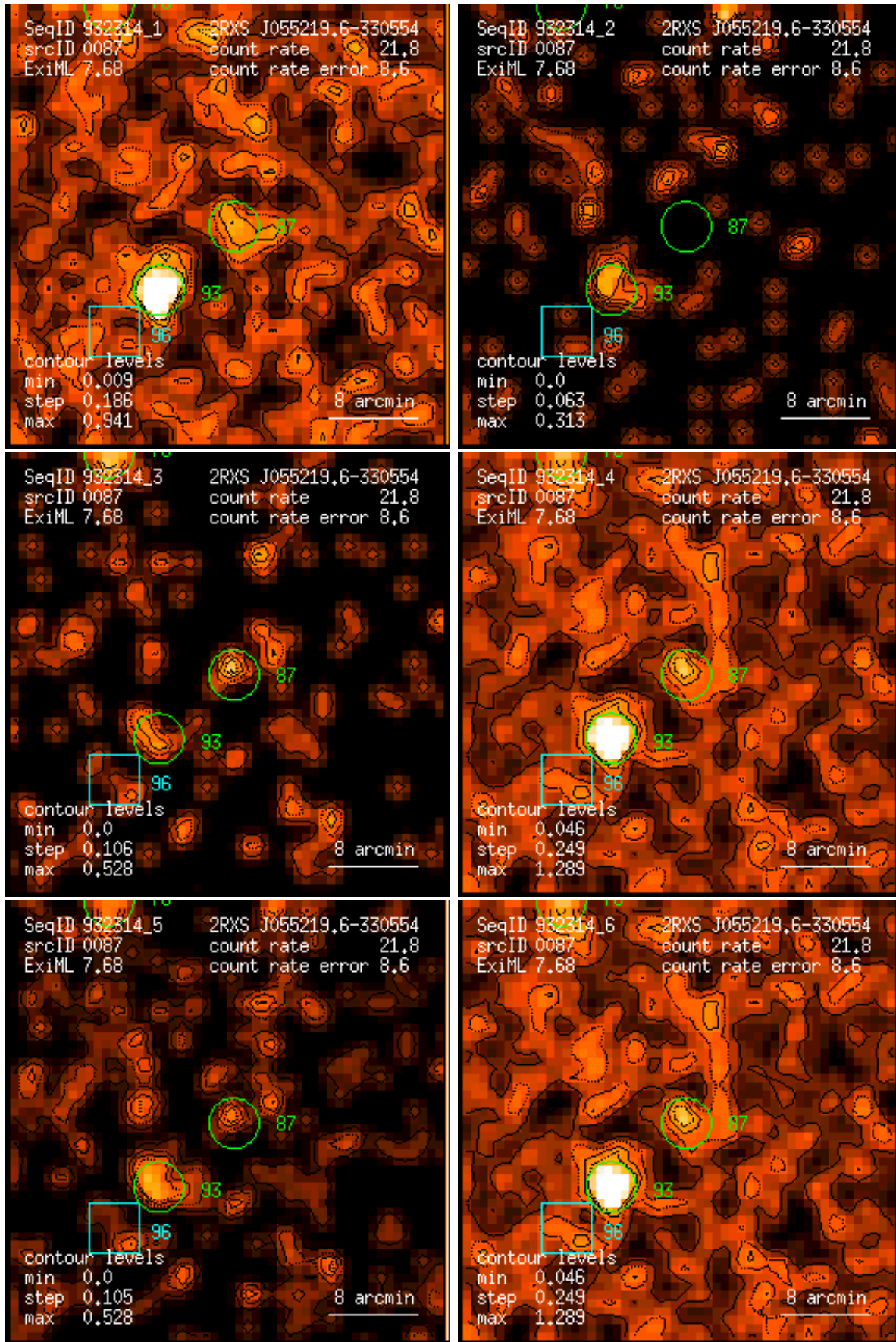
Figure 87: RASS 932314: detection 0087: band rate images, Gaussian filter: (1) PSPC channels 11 – 41, (2) 52 – 90, (3) 91 – 201, (4) 11 – 235, (5) 52 – 201, (6) 11 – 201. Broad band rates in counts/ks. Band rate contour levels in counts/ks/arcmin 2 .
