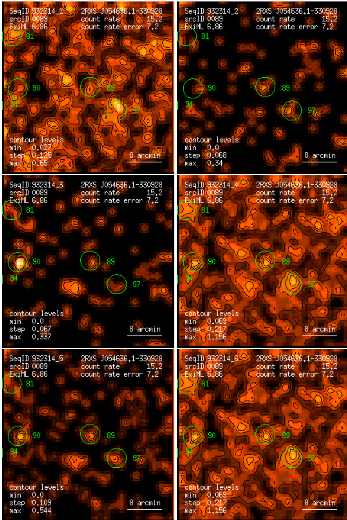
Figure 89: RASS 932314: detection 0089: band rate images, Gaussian filter: (1) PSPC channels 11 – 41, (2) 52 – 90, (3) 91 – 201, (4) 11 – 235, (5) 52 – 201, (6) 11 – 201. Broad band rates in counts/ks. Band rate contour levels in counts/ks/arcmin 2 .
