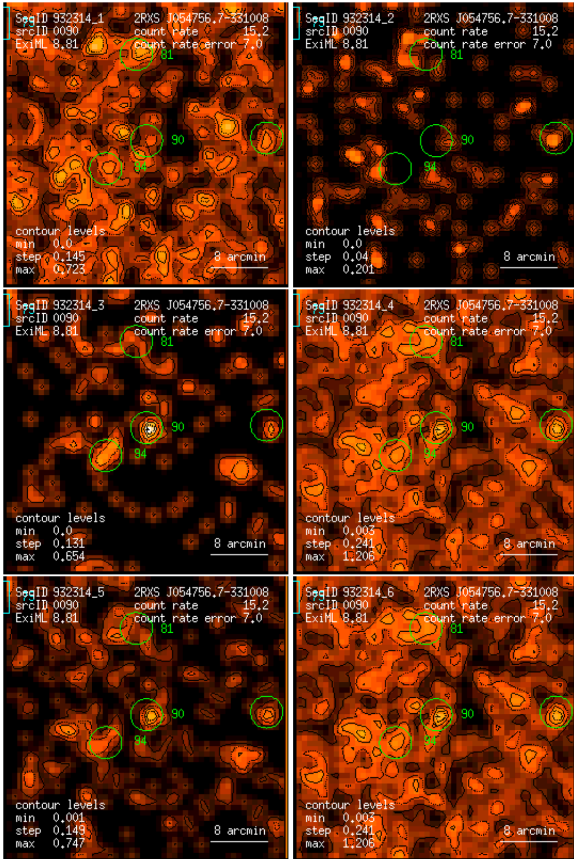
Figure 90: RASS 932314: detection 0090: band rate images, Gaussian filter: (1) PSPC channels 11 – 41, (2) 52 – 90, (3) 91 – 201, (4) 11 – 235, (5) 52 – 201, (6) 11 – 201. Broad band rates in counts/ks. Band rate contour levels in counts/ks/arcmin 2 .
