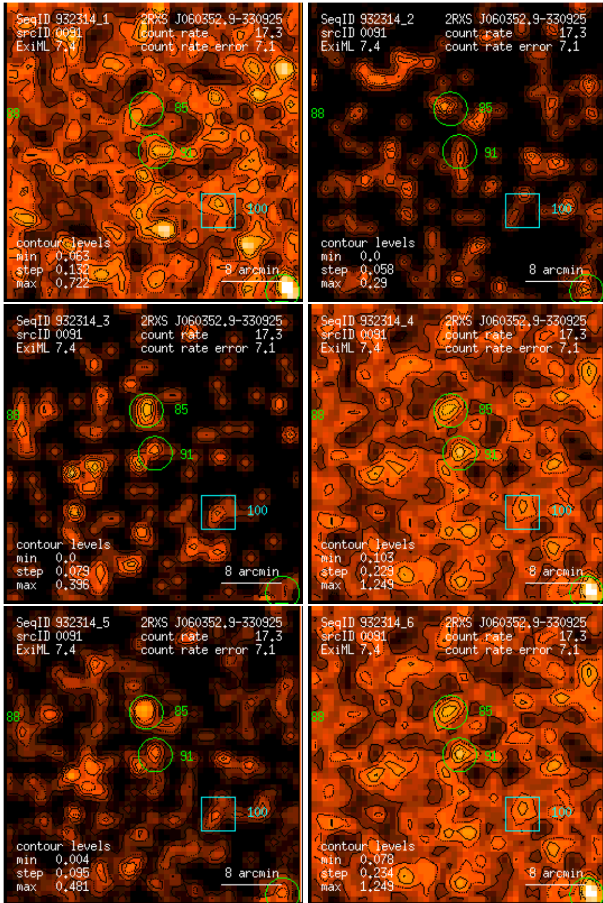
Figure 91: RASS 932314: detection 0091: band rate images, Gaussian filter: (1) PSPC channels 11 – 41, (2) 52 – 90, (3) 91 – 201, (4) 11 – 235, (5) 52 – 201, (6) 11 – 201. Broad band rates in counts/ks. Band rate contour levels in counts/ks/arcmin 2 .
