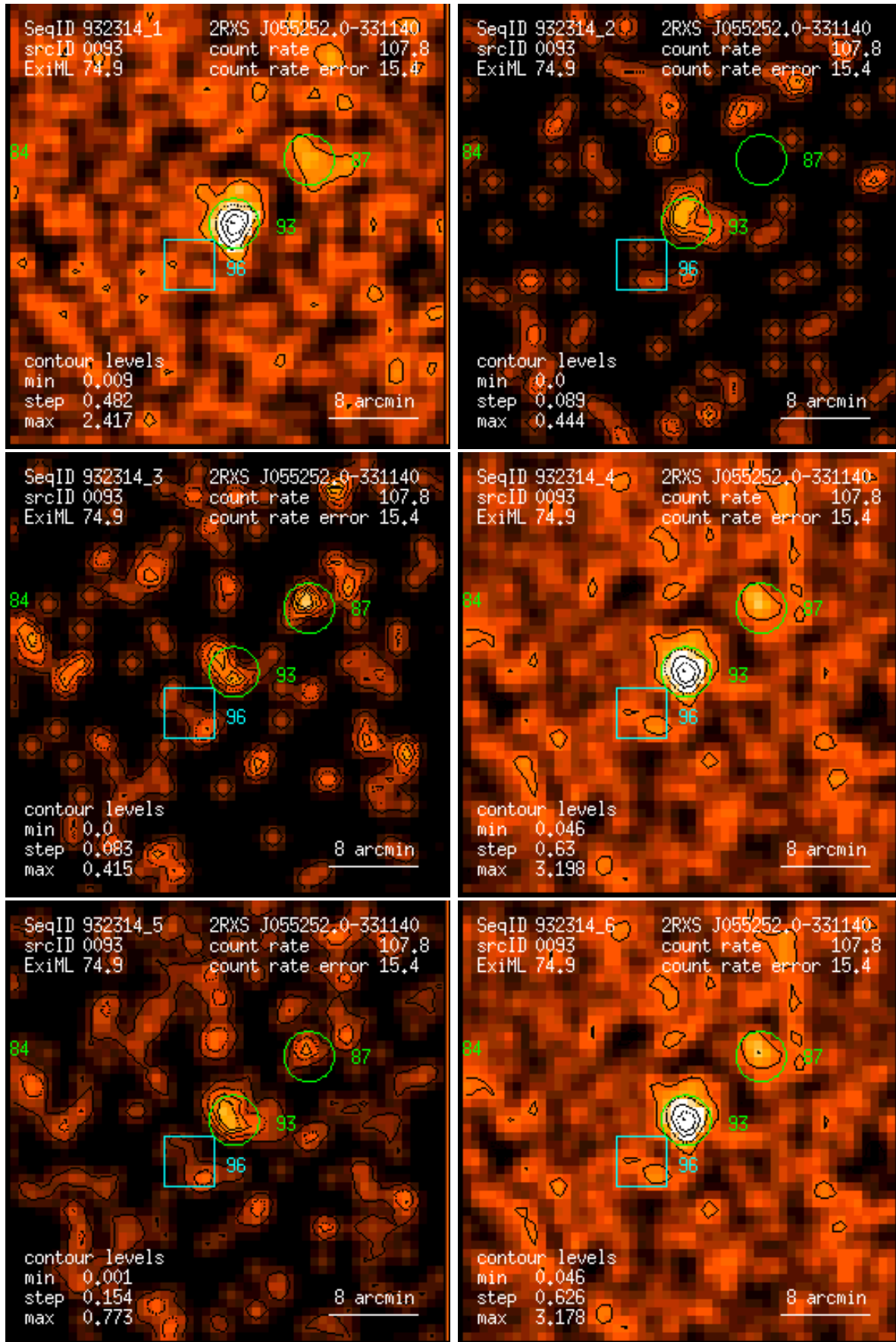
Figure 93: RASS 932314: detection 0093: band rate images, Gaussian filter: (1) PSPC channels 11 – 41, (2) 52 – 90, (3) 91 – 201, (4) 11 – 235, (5) 52 – 201, (6) 11 – 201. Broad band rates in counts/ks. Band rate contour levels in counts/ks/arcmin 2 .
