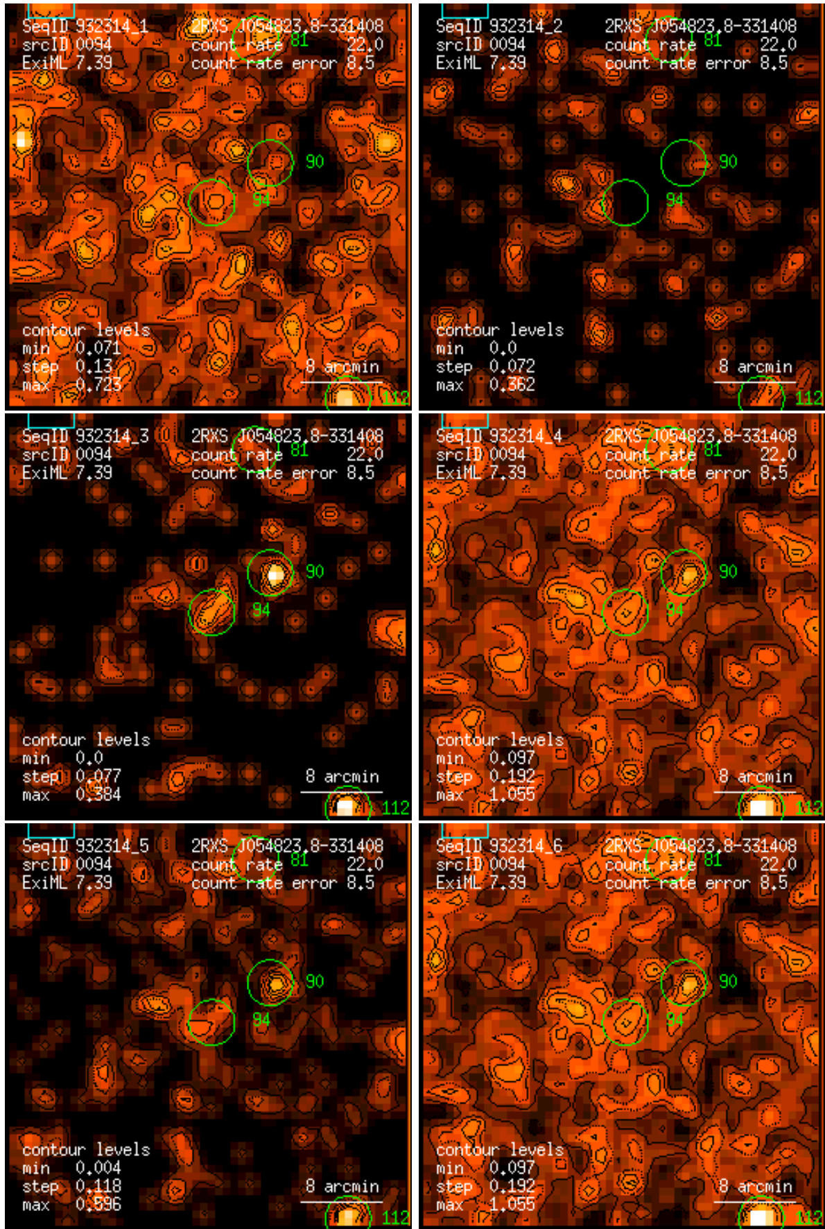
Figure 94: RASS 932314: detection 0094: band rate images, Gaussian filter: (1) PSPC channels 11 – 41, (2) 52 – 90, (3) 91 – 201, (4) 11 – 235, (5) 52 – 201, (6) 11 – 201. Broad band rates in counts/ks. Band rate contour levels in counts/ks/arcmin 2 .
