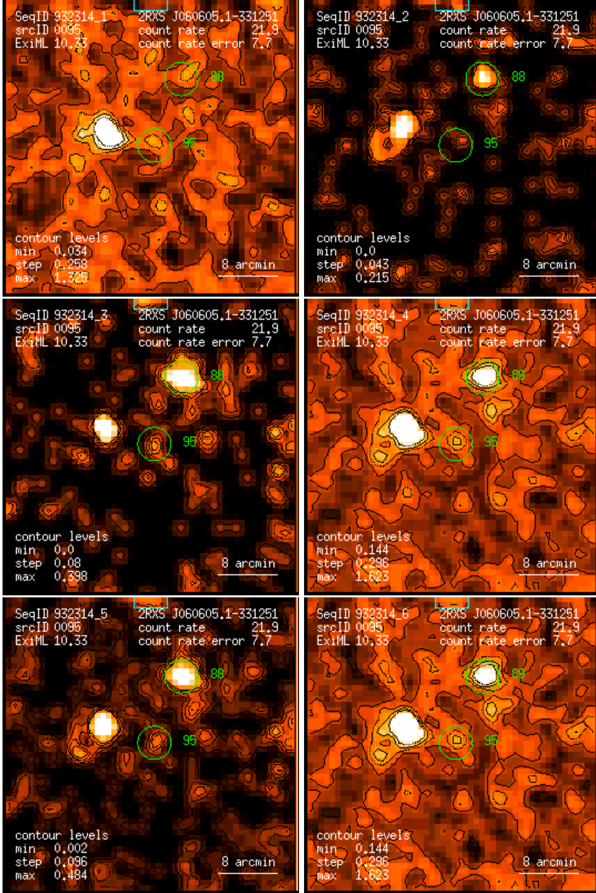
Figure 95: RASS 932314: detection 0095: band rate images, Gaussian filter: (1) PSPC channels 11 – 41, (2) 52 – 90, (3) 91 – 201, (4) 11 – 235, (5) 52 – 201, (6) 11 – 201. Broad band rates in counts/ks. Band rate contour levels in counts/ks/arcmin 2 .
