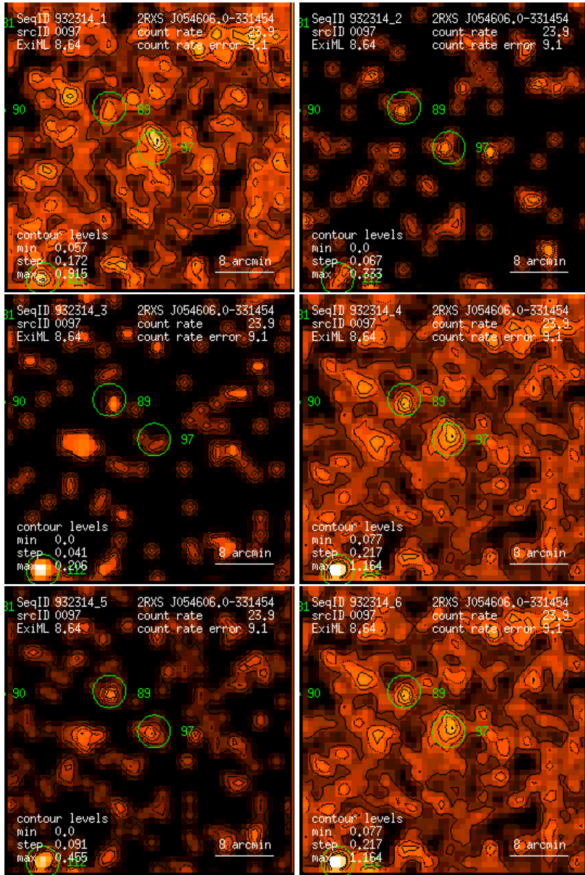
Figure 97: RASS 932314: detection 0097: band rate images, Gaussian filter: (1) PSPC channels 11 – 41, (2) 52 – 90, (3) 91 – 201, (4) 11 – 235, (5) 52 – 201, (6) 11 – 201. Broad band rates in counts/ks. Band rate contour levels in counts/ks/arcmin 2 .
