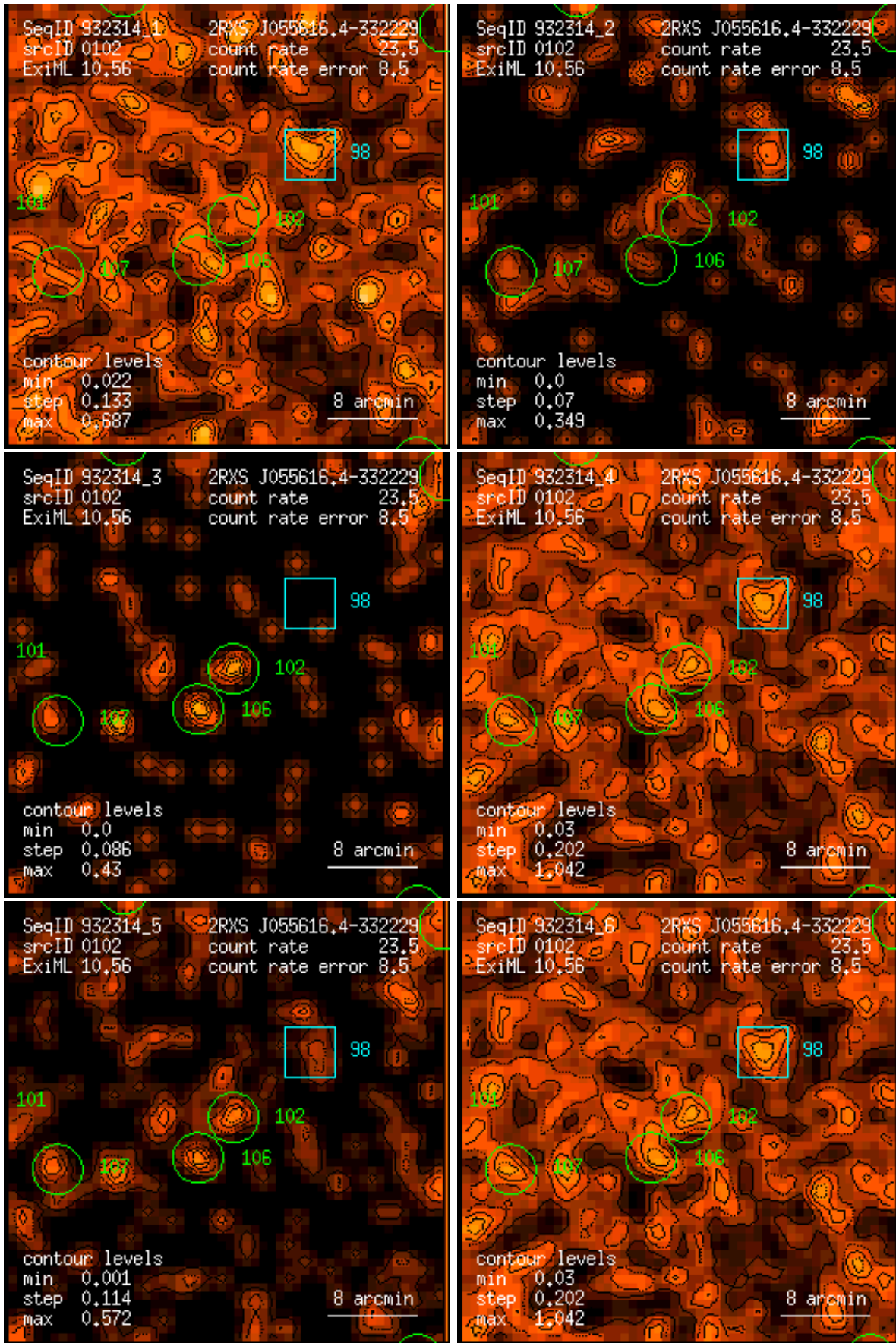
Figure 102: RASS 932314: detection 0102: band rate images, Gaussian filter: (1) PSPC channels 11 – 41, (2) 52 – 90, (3) 91 – 201, (4) 11 – 235, (5) 52 – 201, (6) 11 – 201. Broad band rates in counts/ks. Band rate contour levels in counts/ks/arcmin 2 .
