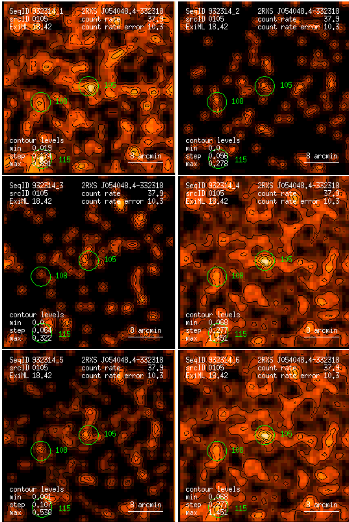
Figure 105: RASS 932314: detection 0105: band rate images, Gaussian filter: (1) PSPC channels 11 – 41, (2) 52 – 90, (3) 91 – 201, (4) 11 – 235, (5) 52 – 201, (6) 11 – 201. Broad band rates in counts/ks. Band rate contour levels in counts/ks/arcmin 2 .
