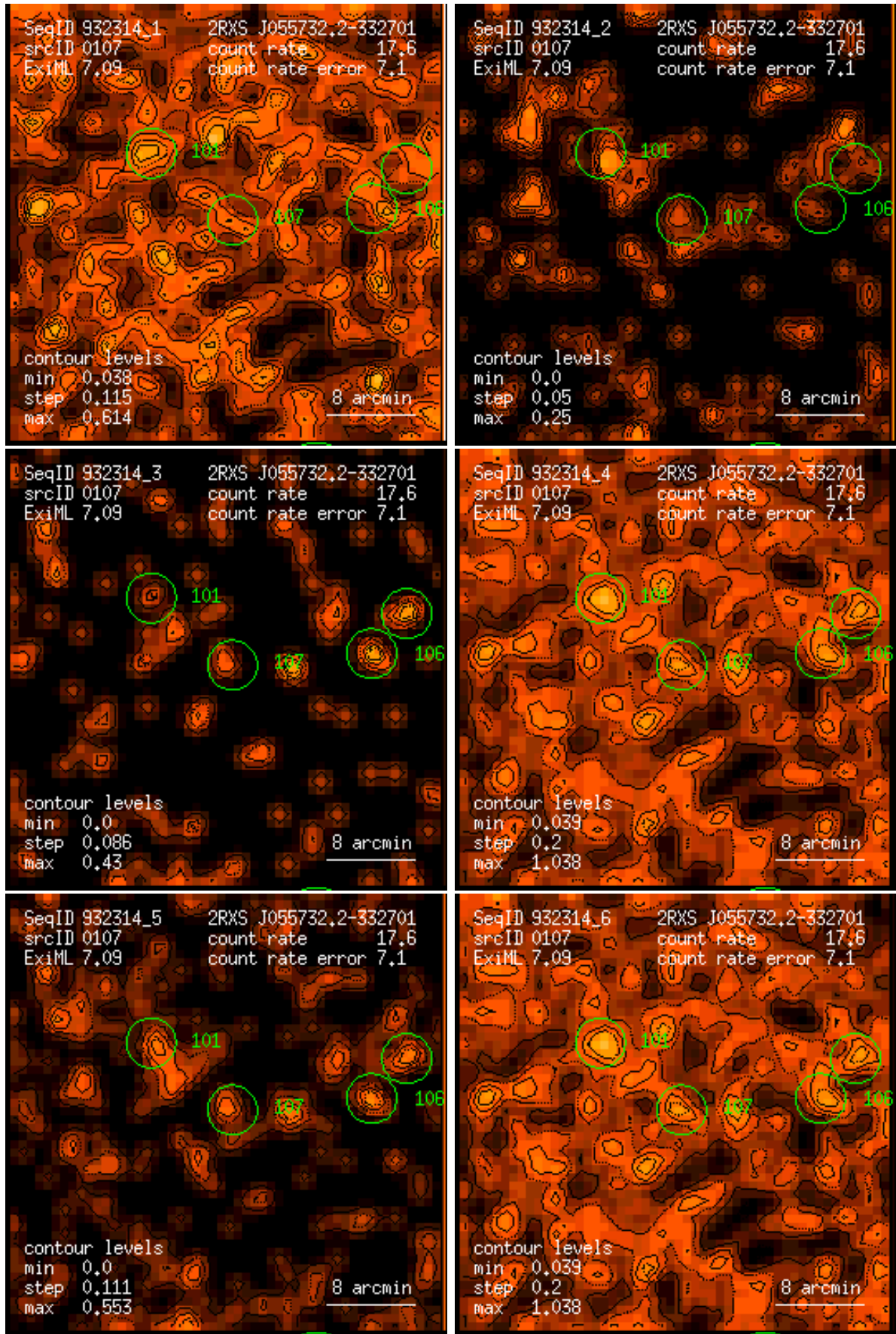
Figure 107: RASS 932314: detection 0107: band rate images, Gaussian filter: (1) PSPC channels 11 – 41, (2) 52 – 90, (3) 91 – 201, (4) 11 – 235, (5) 52 – 201, (6) 11 – 201. Broad band rates in counts/ks. Band rate contour levels in counts/ks/arcmin 2 .
