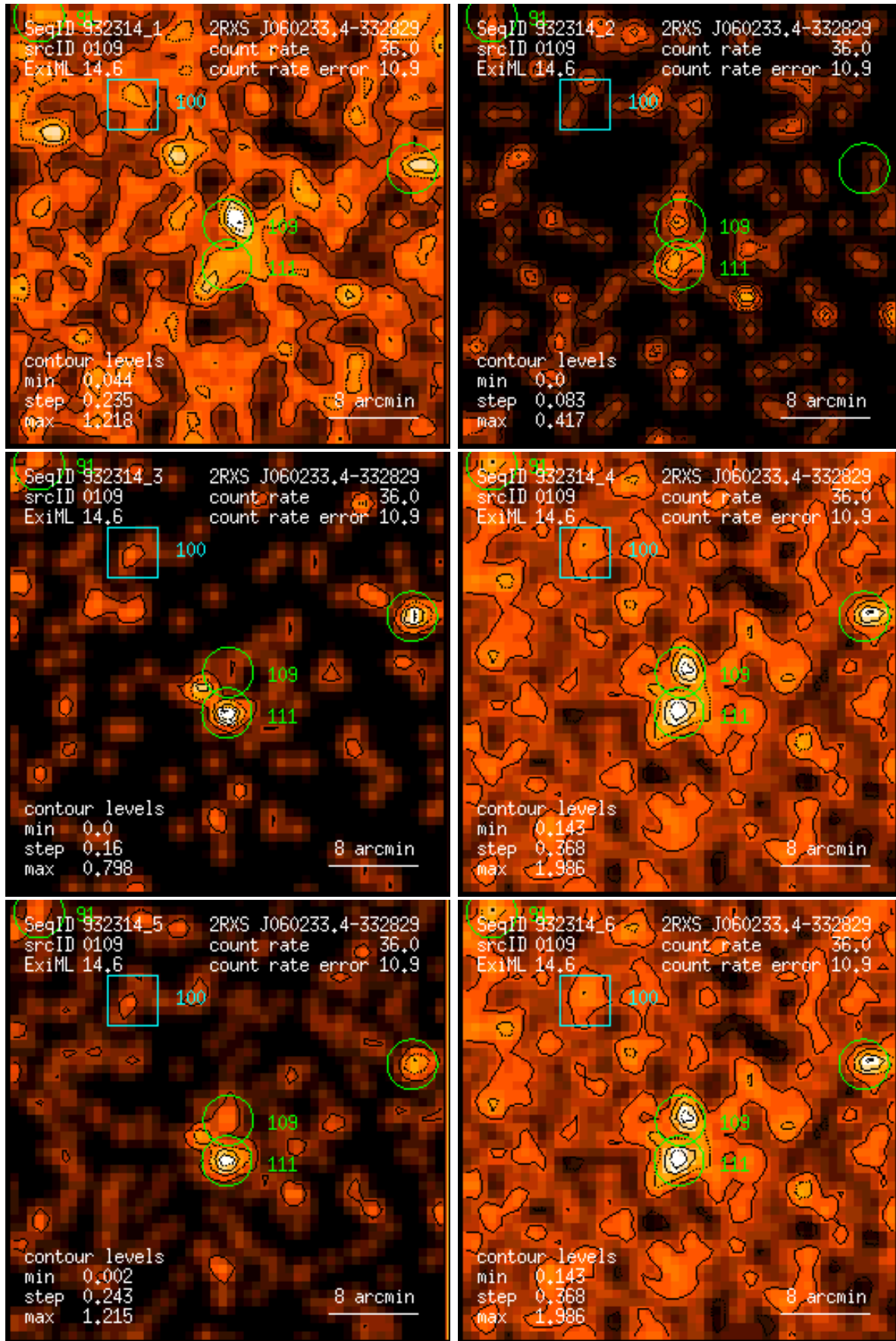
Figure 109: RASS 932314: detection 0109: band rate images, Gaussian filter: (1) PSPC channels 11 – 41, (2) 52 – 90, (3) 91 – 201, (4) 11 – 235, (5) 52 – 201, (6) 11 – 201. Broad band rates in counts/ks. Band rate contour levels in counts/ks/arcmin 2 .
