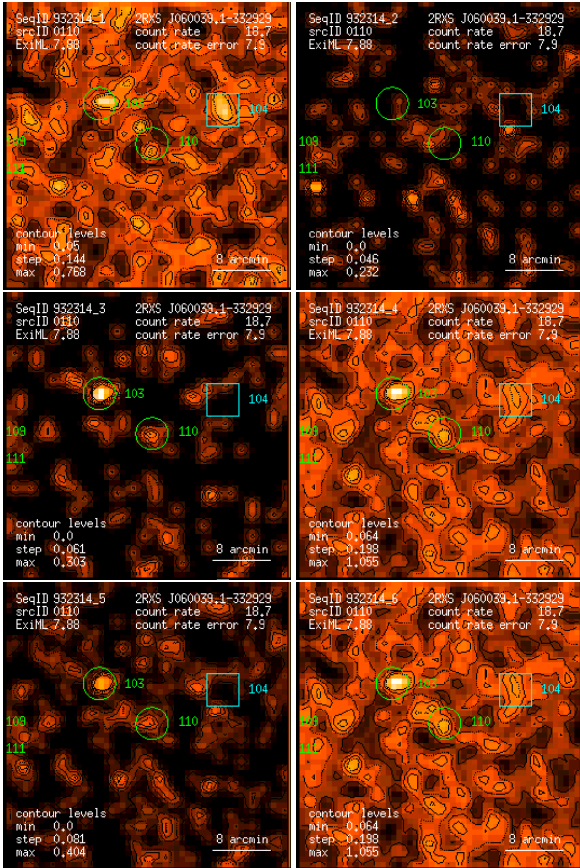
Figure 110: RASS 932314: detection 0110: band rate images, Gaussian filter: (1) PSPC channels 11 – 41, (2) 52 – 90, (3) 91 – 201, (4) 11 – 235, (5) 52 – 201, (6) 11 – 201. Broad band rates in counts/ks. Band rate contour levels in counts/ks/arcmin 2 .
