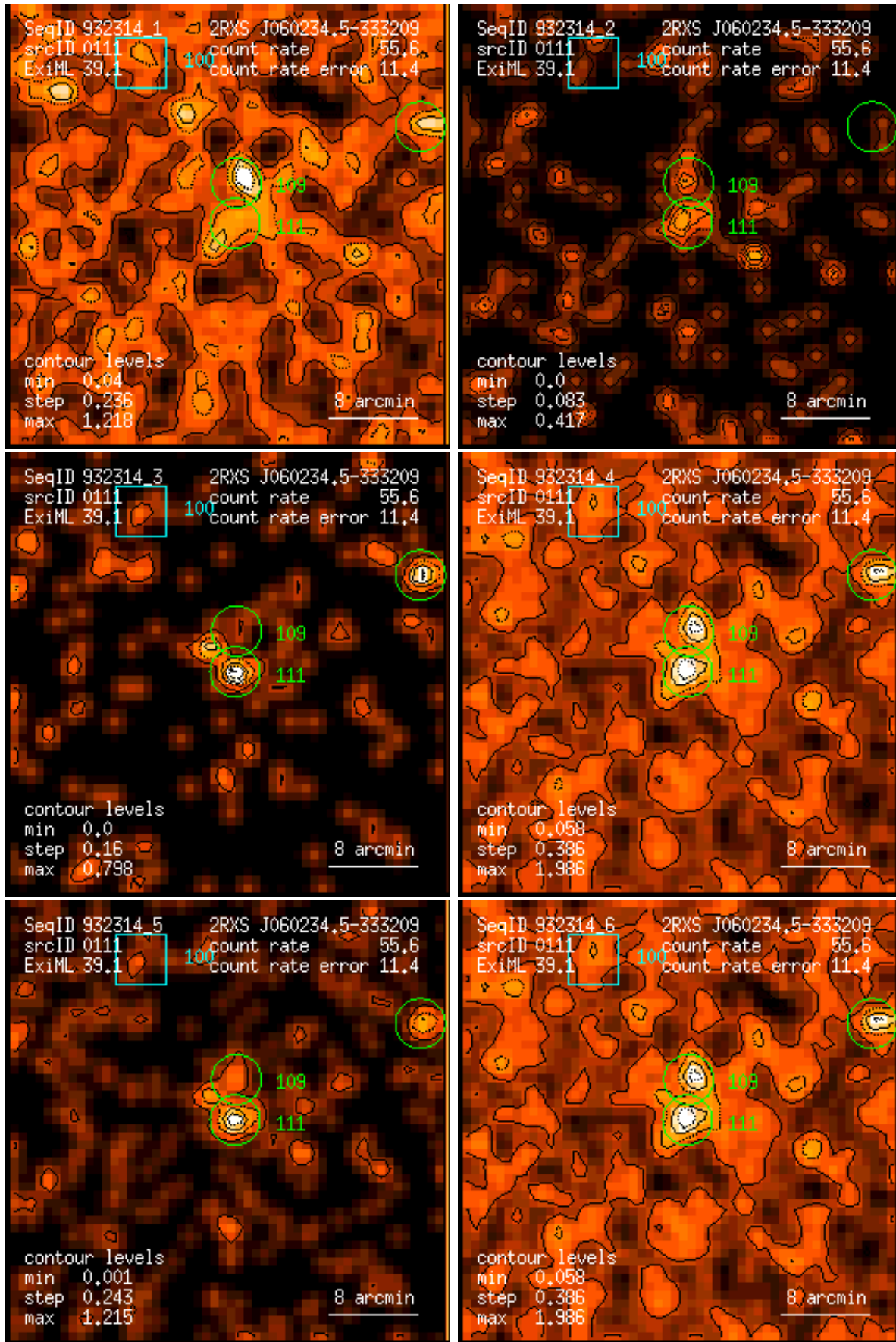
Figure 111: RASS 932314: detection 0111: band rate images, Gaussian filter: (1) PSPC channels 11 – 41, (2) 52 – 90, (3) 91 – 201, (4) 11 – 235, (5) 52 – 201, (6) 11 – 201. Broad band rates in counts/ks. Band rate contour levels in counts/ks/arcmin 2 .
