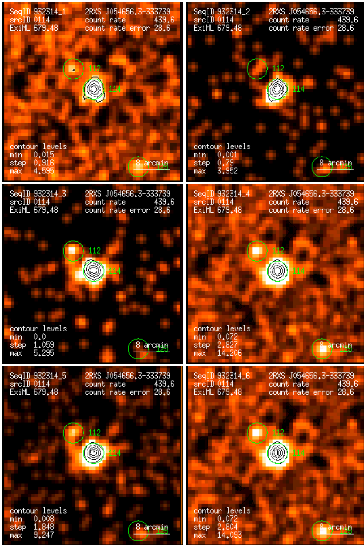
Figure 114: RASS 932314: detection 0114: band rate images, Gaussian filter: (1) PSPC channels 11 – 41, (2) 52 – 90, (3) 91 – 201, (4) 11 – 235, (5) 52 – 201, (6) 11 – 201. Broad band rates in counts/ks. Band rate contour levels in counts/ks/arcmin 2 .
