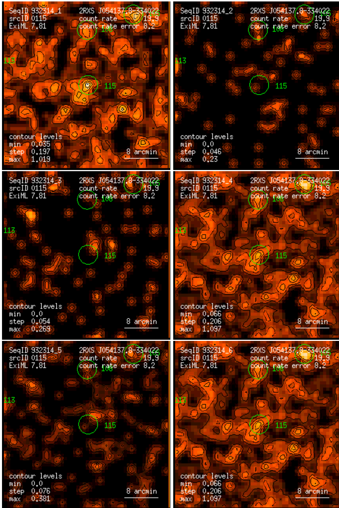
Figure 115: RASS 932314: detection 0115: band rate images, Gaussian filter: (1) PSPC channels 11 – 41, (2) 52 – 90, (3) 91 – 201, (4) 11 – 235, (5) 52 – 201, (6) 11 – 201. Broad band rates in counts/ks. Band rate contour levels in counts/ks/arcmin 2 .
