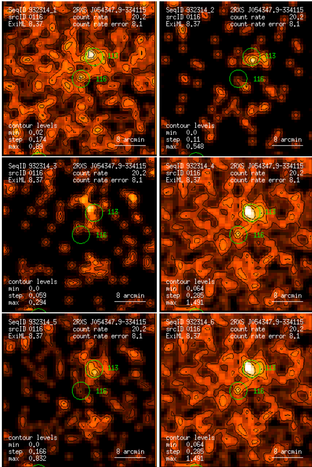
Figure 116: RASS 932314: detection 0116: band rate images, Gaussian filter: (1) PSPC channels 11 – 41, (2) 52 – 90, (3) 91 – 201, (4) 11 – 235, (5) 52 – 201, (6) 11 – 201. Broad band rates in counts/ks. Band rate contour levels in counts/ks/arcmin 2 .
