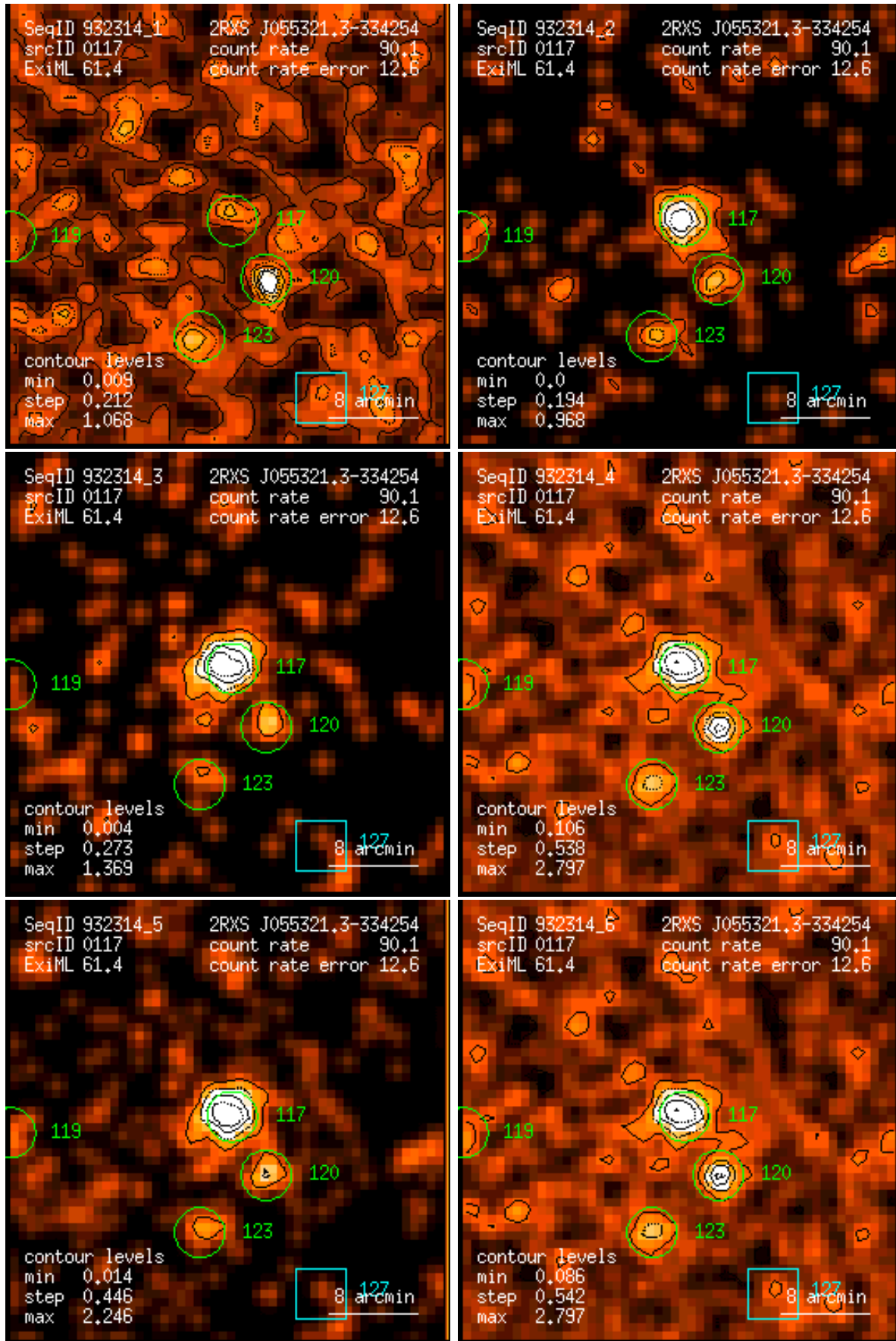
Figure 117: RASS 932314: detection 0117: band rate images, Gaussian filter: (1) PSPC channels 11 – 41, (2) 52 – 90, (3) 91 – 201, (4) 11 – 235, (5) 52 – 201, (6) 11 – 201. Broad band rates in counts/ks. Band rate contour levels in counts/ks/arcmin 2 .
