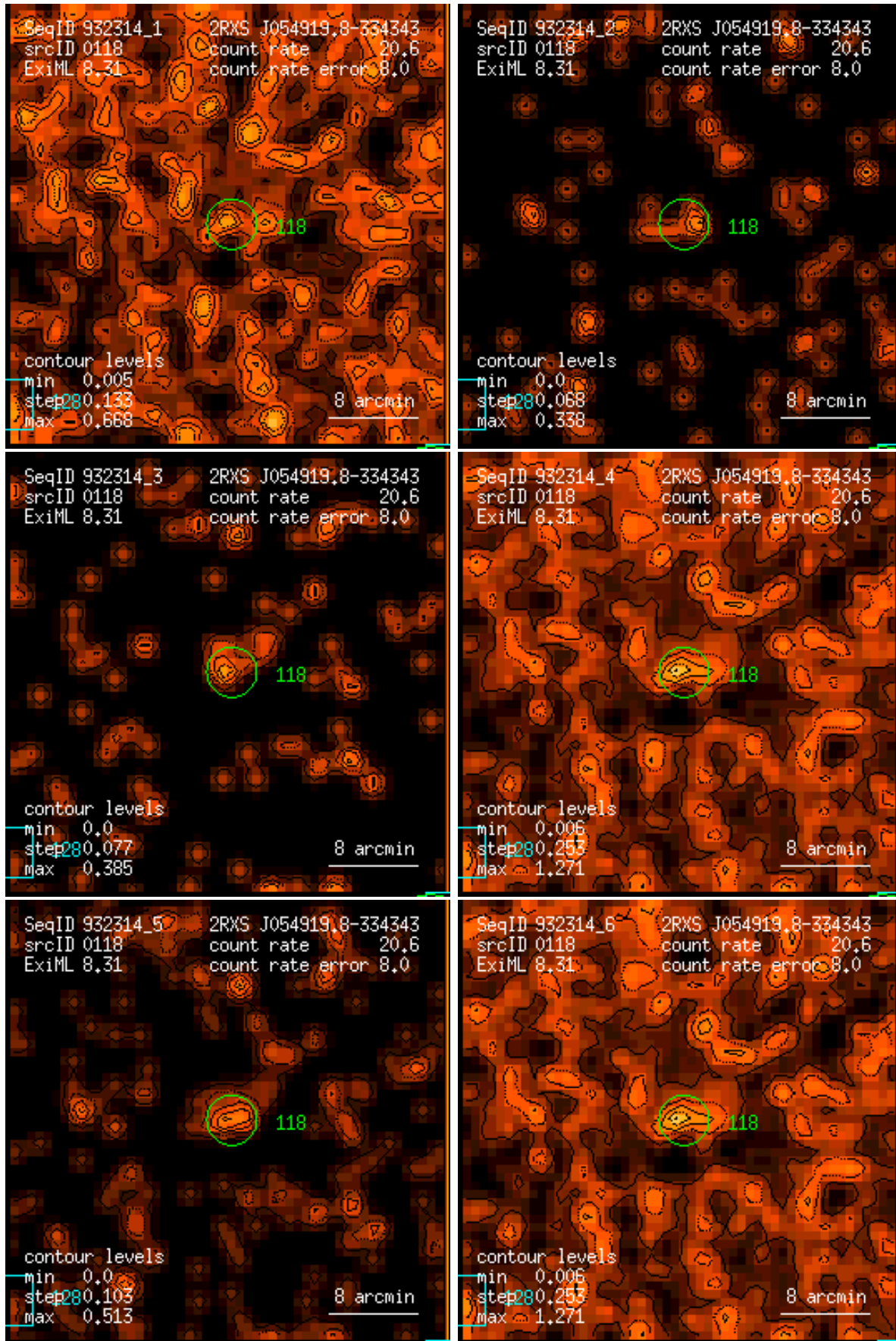
Figure 118: RASS 932314: detection 0118: band rate images, Gaussian filter: (1) PSPC channels 11 – 41, (2) 52 – 90, (3) 91 – 201, (4) 11 – 235, (5) 52 – 201, (6) 11 – 201. Broad band rates in counts/ks. Band rate contour levels in counts/ks/arcmin 2 .
