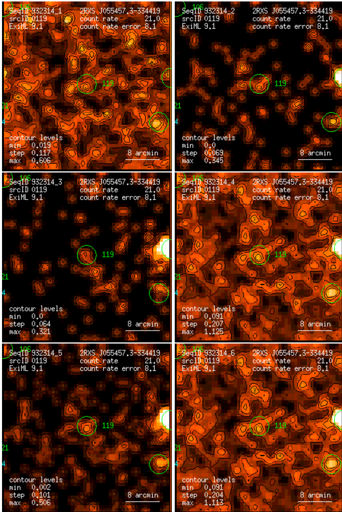
Figure 119: RASS 932314: detection 0119: band rate images, Gaussian filter: (1) PSPPC channels 11 – 41, (2) 52 – 90, (3) 91 – 201, (4) 11 – 235, (5) 52 – 201, (6) 11 – 201. Broad band rates in counts/ks. Band rate contour levels in counts/ks/arcmin 2 .
