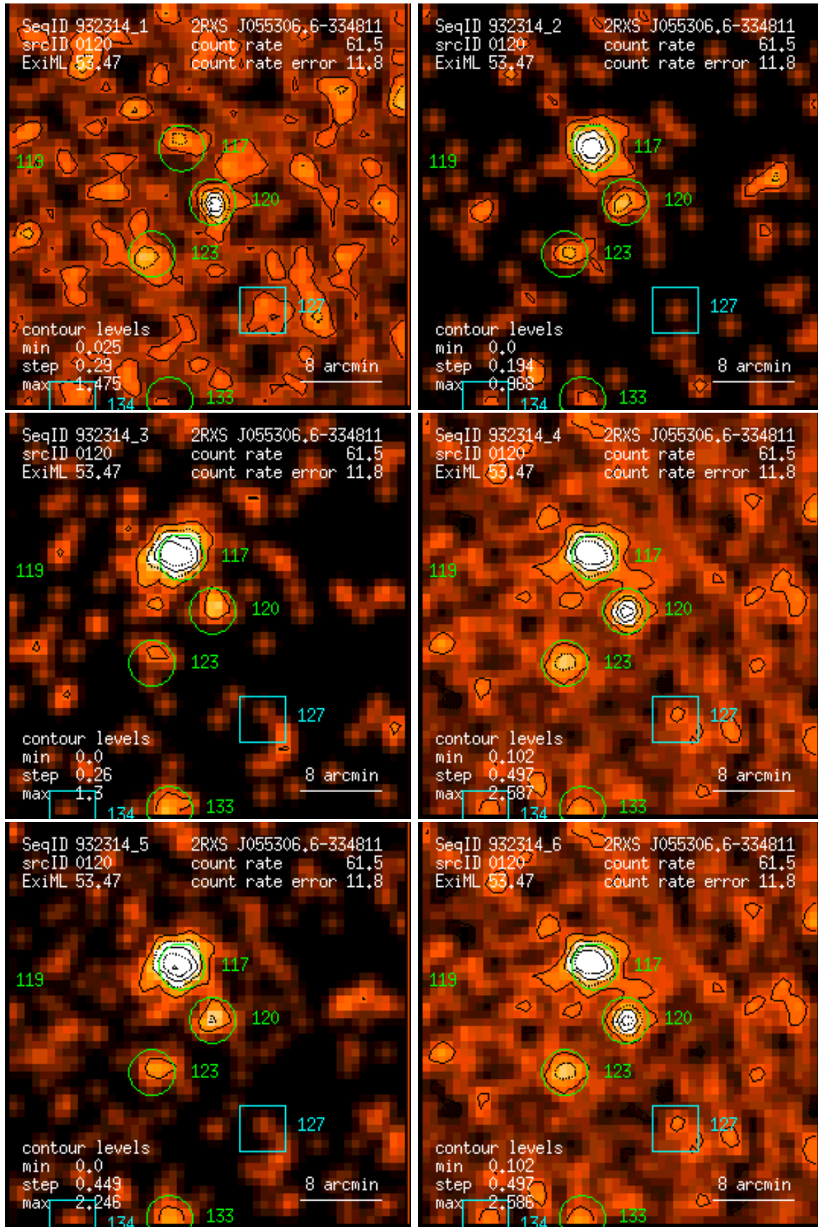
Figure 120: RASS 932314: detection 0120: band rate images, Gaussian filter: (1) PSPC channels 11 – 41, (2) 52 – 90, (3) 91 – 201, (4) 11 – 235, (5) 52 – 201, (6) 11 – 201. Broad band rates in counts/ks. Band rate contour levels in counts/ks/arcmin 2 .
