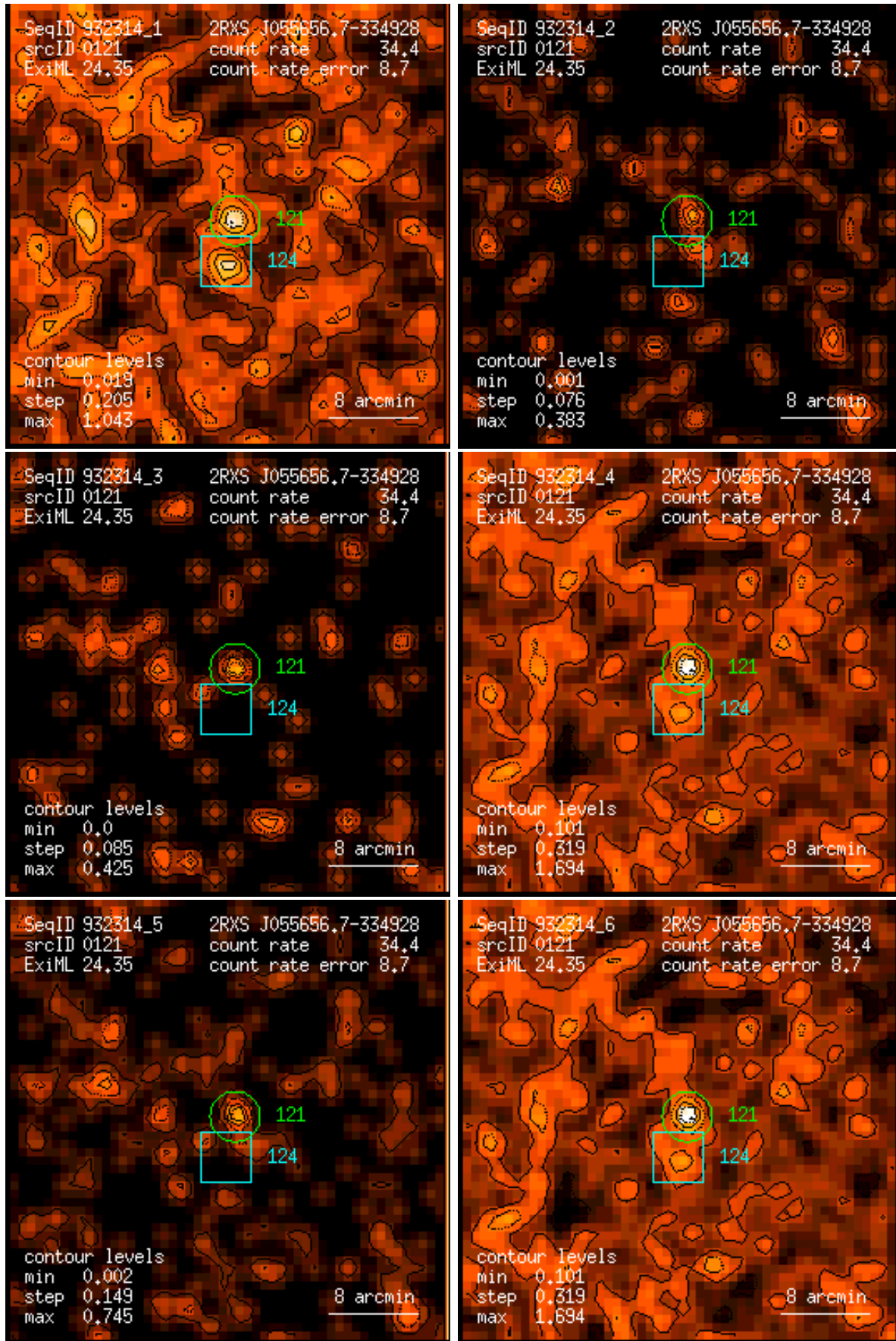
Figure 121: RASS 932314: detection 0121: band rate images, Gaussian filter: (1) PSPC channels 11 – 41, (2) 52 – 90, (3) 91 – 201, (4) 11 – 235, (5) 52 – 201, (6) 11 – 201. Broad band rates in counts/ks. Band rate contour levels in counts/ks/arcmin 2 .
