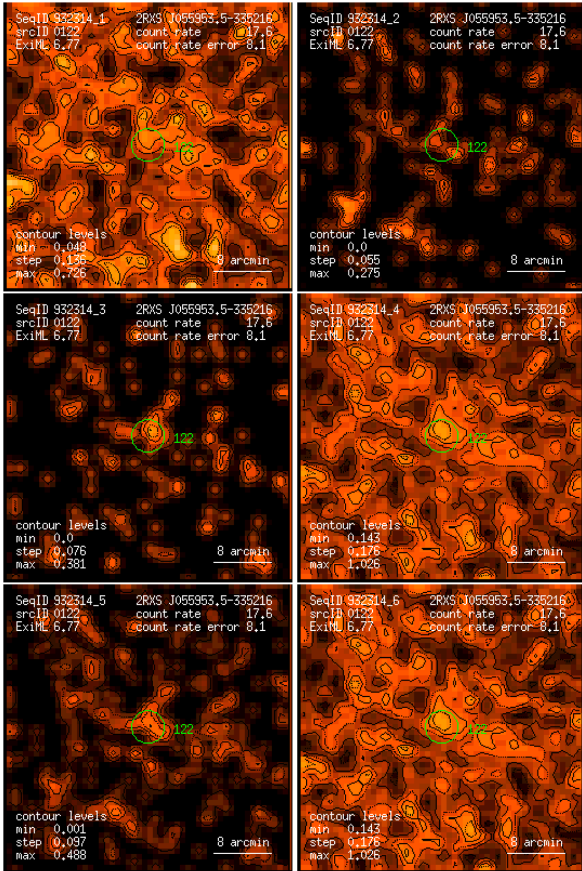
Figure 122: RASS 932314: detection 0122: band rate images, Gaussian filter: (1) PSPC channels 11 – 41, (2) 52 – 90, (3) 91 – 201, (4) 11 – 235, (5) 52 – 201, (6) 11 – 201. Broad band rates in counts/ks. Band rate contour levels in counts/ks/arcmin 2 .
