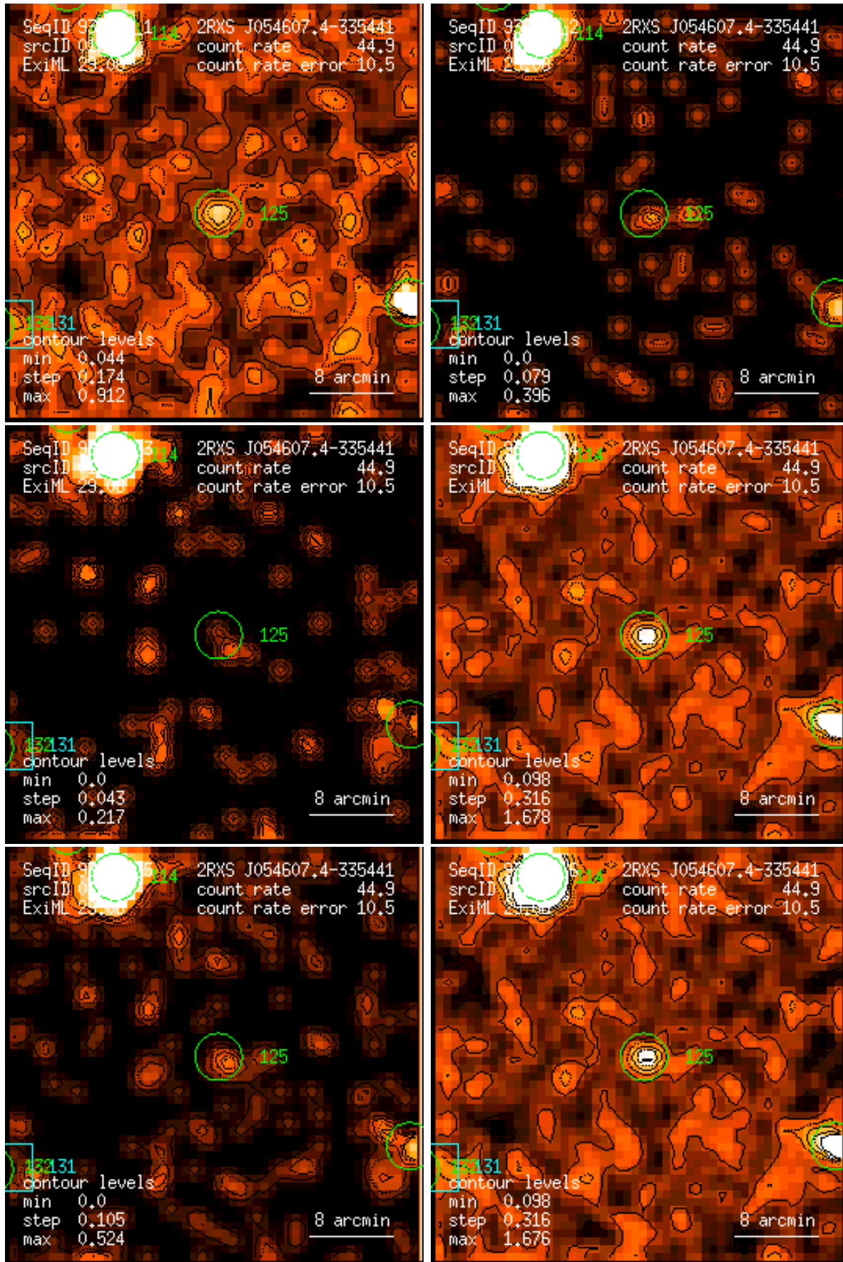
Figure 125: RASS 932314: detection 0125: band rate images, Gaussian filter: (1) PSPC channels 11 – 41, (2) 52 – 90, (3) 91 – 201, (4) 11 – 235, (5) 52 – 201, (6) 11 – 201. Broad band rates in counts/ks. Band rate contour levels in counts/ks/arcmin 2 .
