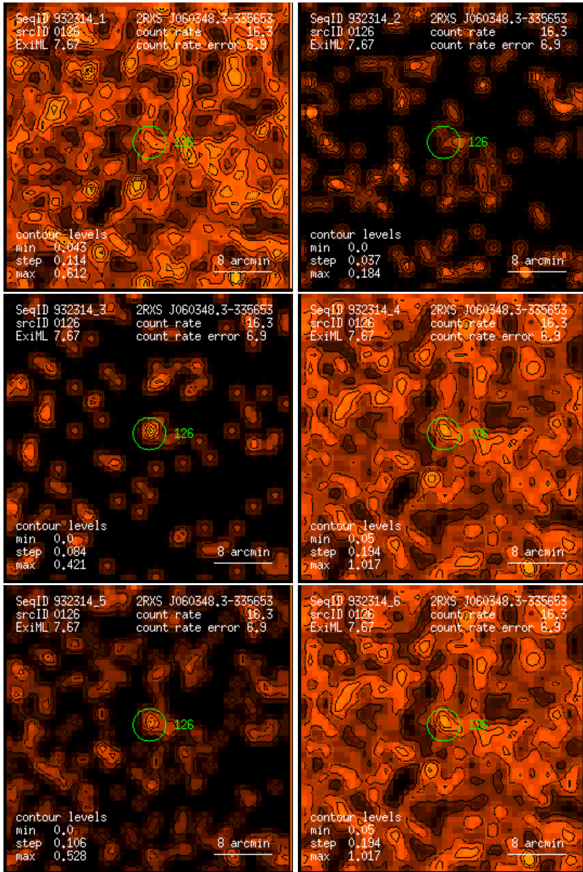
Figure 126: RASS 932314: detection 0126: band rate images, Gaussian filter: (1) PSPC channels 11 – 41, (2) 52 – 90, (3) 91 – 201, (4) 11 – 235, (5) 52 – 201, (6) 11 – 201. Broad band rates in counts/ks. Band rate contour levels in counts/ks/arcmin 2 .
