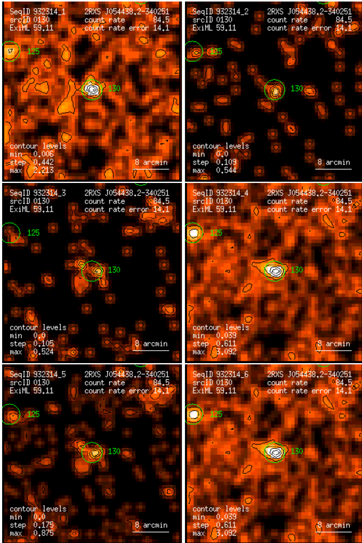
Figure 130: RASS 932314: detection 0130: band rate images, Gaussian filter: (1) PSPC channels 11 – 41, (2) 52 – 90, (3) 91 – 201, (4) 11 – 235, (5) 52 – 201, (6) 11 – 201. Broad band rates in counts/ks. Band rate contour levels in counts/ks/arcmin 2 .
