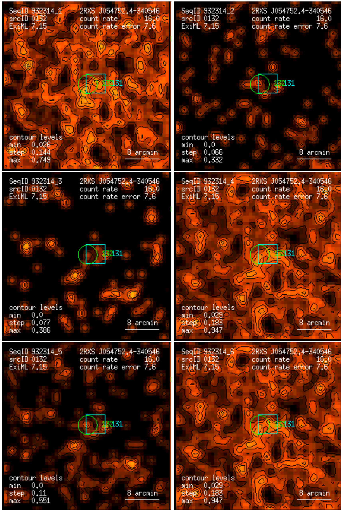
Figure 132: RASS 932314: detection 0132: band rate images, Gaussian filter: (1) PSPC channels 11 – 41, (2) 52 – 90, (3) 91 – 201, (4) 11 – 235, (5) 52 – 201, (6) 11 – 201. Broad band rates in counts/ks. Band rate contour levels in counts/ks/arcmin 2 .
