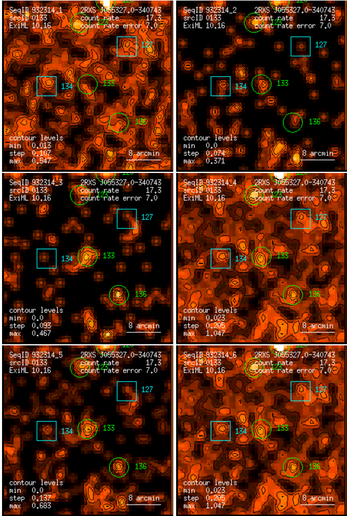
Figure 133: RASS 932314: detection 0133: band rate images, Gaussian filter: (1) PSPC channels 11 – 41, (2) 52 – 90, (3) 91 – 201, (4) 11 – 235, (5) 52 – 201, (6) 11 – 201. Broad band rates in counts/ks. Band rate contour levels in counts/ks/arcmin 2 .
