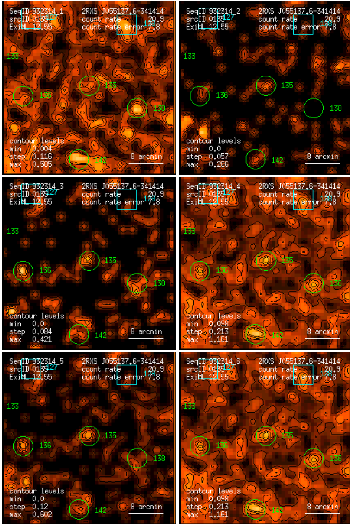
Figure 135: RASS 932314: detection 0135: band rate images, Gaussian filter: (1) PSPC channels 11 – 41, (2) 52 – 90, (3) 91 – 201, (4) 11 – 235, (5) 52 – 201, (6) 11 – 201. Broad band rates in counts/ks. Band rate contour levels in counts/ks/arcmin 2 .
