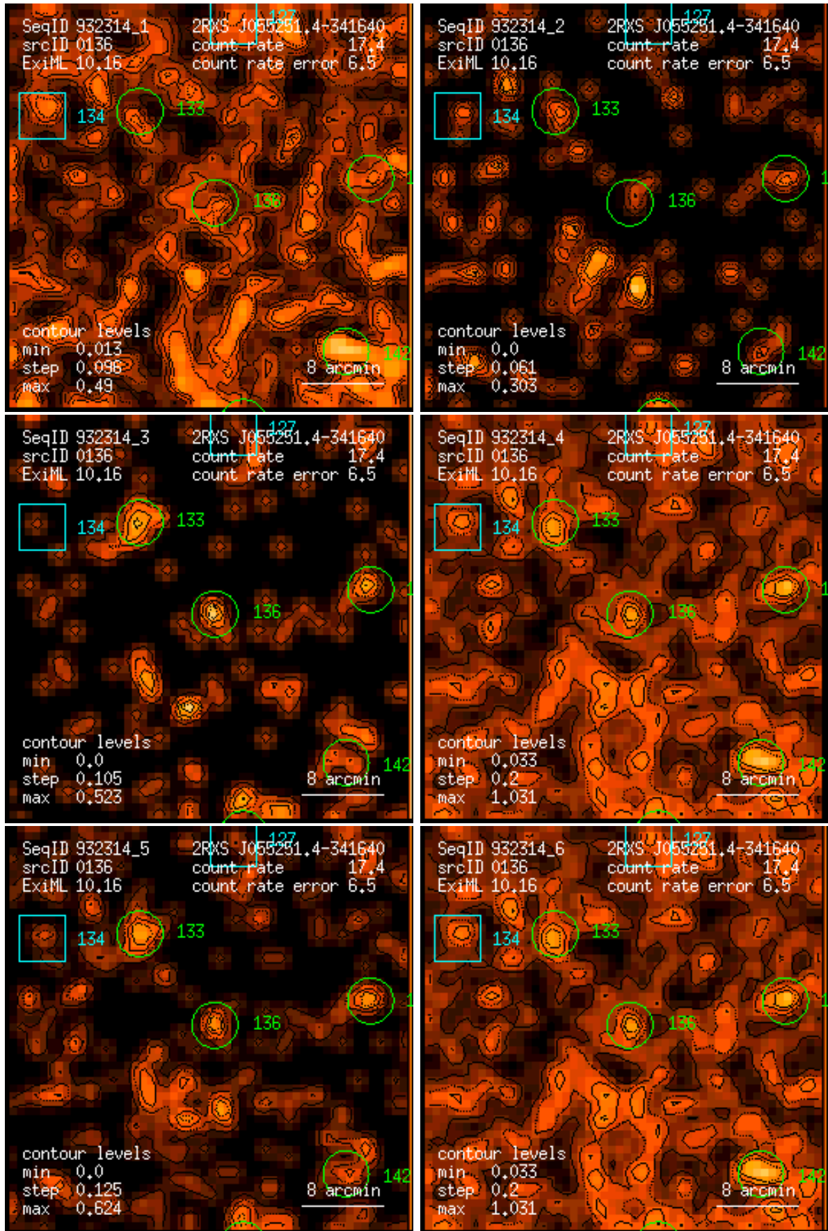
Figure 136: RASS 932314: detection 0136: band rate images, Gaussian filter: (1) PSPC channels 11 – 41, (2) 52 – 90, (3) 91 – 201, (4) 11 – 235, (5) 52 – 201, (6) 11 – 201. Broad band rates in counts/ks. Band rate contour levels in counts/ks/arcmin 2 .
