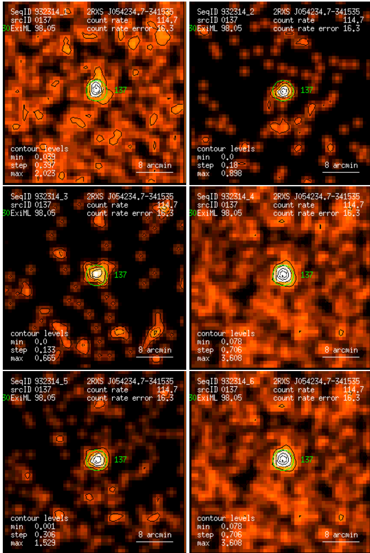
Figure 137: RASS 932314: detection 0137: band rate images, Gaussian filter: (1) PSPC channels 11 – 41, (2) 52 – 90, (3) 91 – 201, (4) 11 – 235, (5) 52 – 201, (6) 11 – 201. Broad band rates in counts/ks. Band rate contour levels in counts/ks/arcmin 2 .
