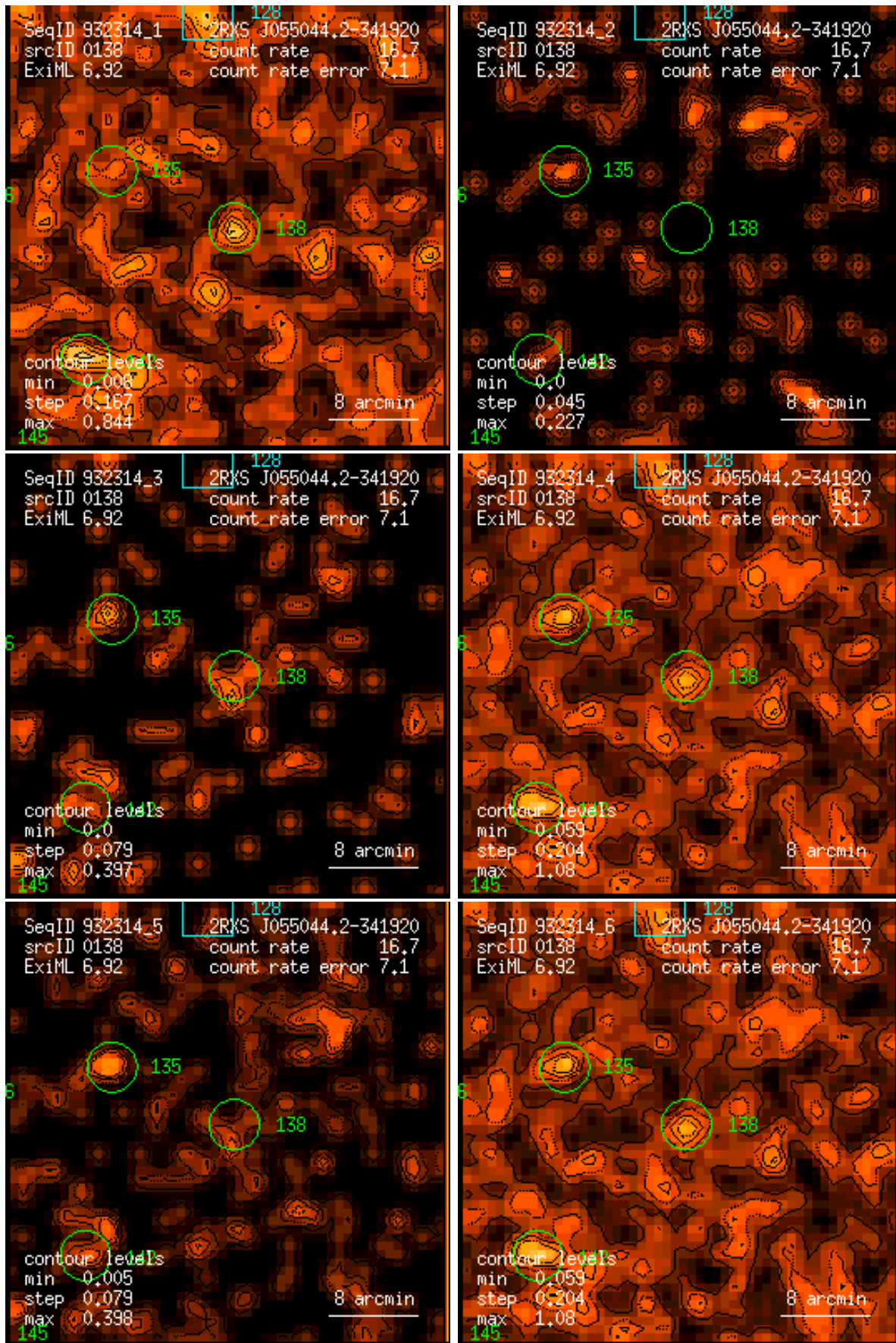
Figure 138: RASS 932314: detection 0138: band rate images, Gaussian filter: (1) PSPC channels 11 – 41, (2) 52 – 90, (3) 91 – 201, (4) 11 – 235, (5) 52 – 201, (6) 11 – 201. Broad band rates in counts/ks. Band rate contour levels in counts/ks/arcmin 2 .
