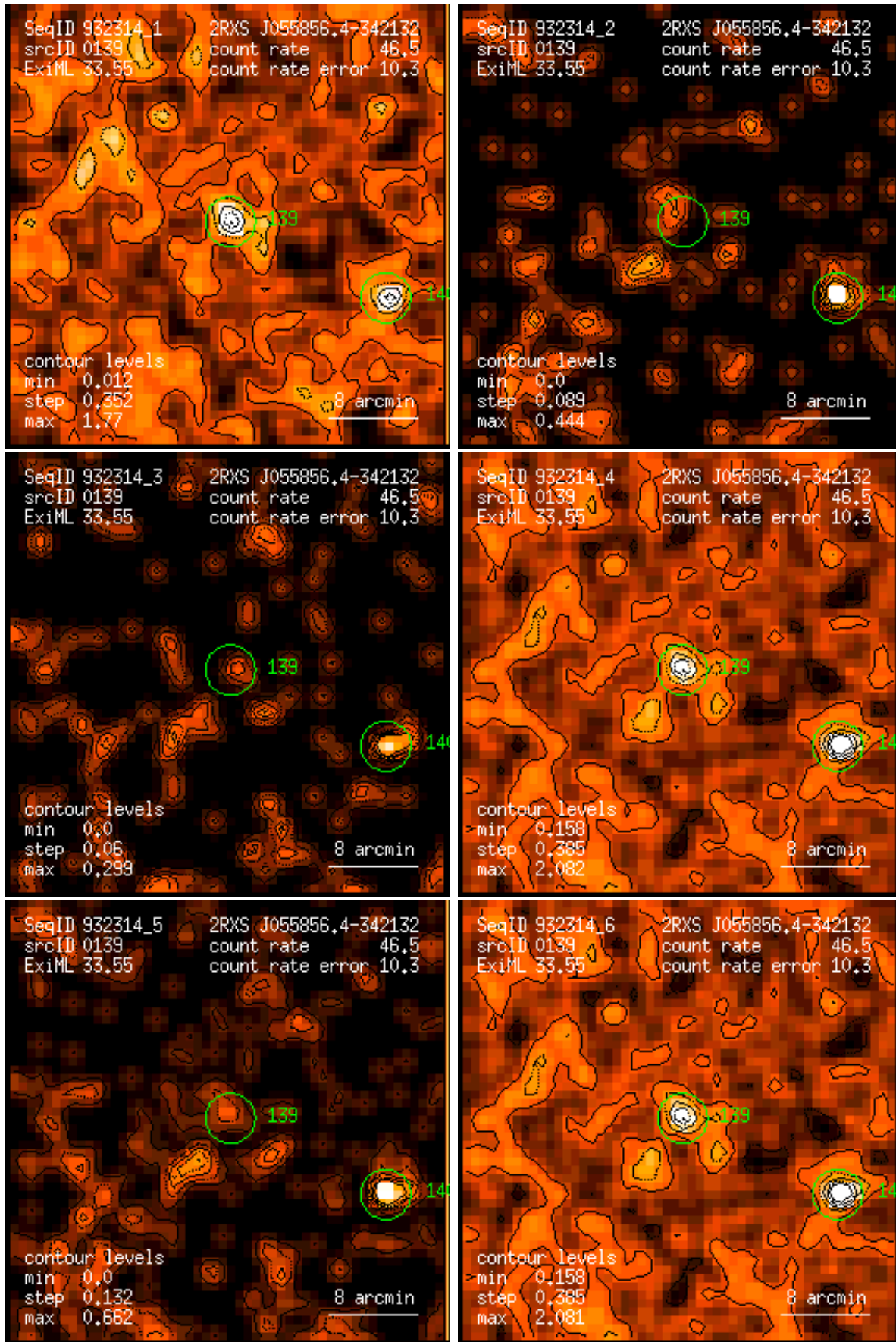
Figure 139: RASS 932314: detection 0139: band rate images, Gaussian filter: (1) PSPC channels 11 – 41, (2) 52 – 90, (3) 91 – 201, (4) 11 – 235, (5) 52 – 201, (6) 11 – 201. Broad band rates in counts/ks. Band rate contour levels in counts/ks/arcmin 2 .
