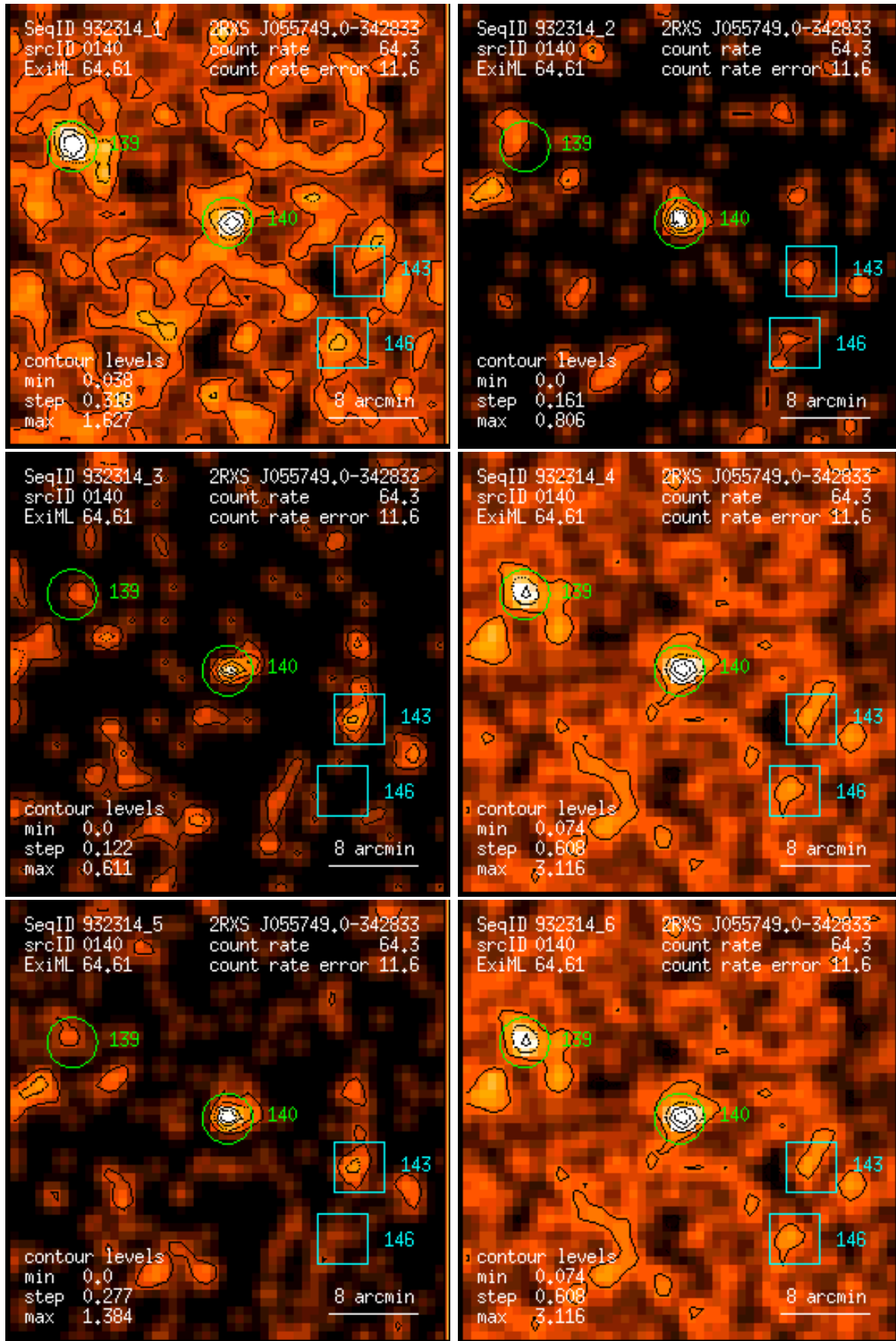
Figure 140: RASS 932314: detection 0140: band rate images, Gaussian filter: (1) PSPC channels 11 – 41, (2) 52 – 90, (3) 91 – 201, (4) 11 – 235, (5) 52 – 201, (6) 11 – 201. Broad band rates in counts/ks. Band rate contour levels in counts/ks/arcmin 2 .
