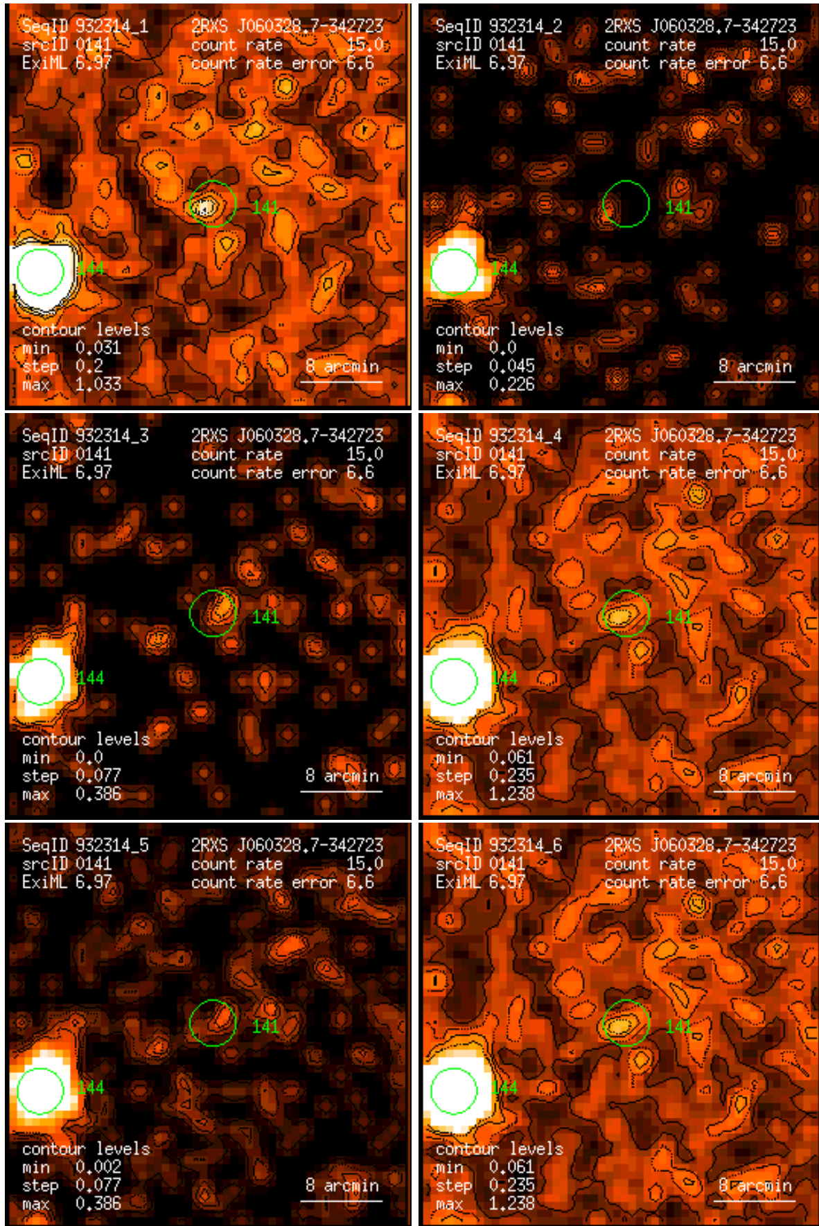
Figure 141: RASS 932314: detection 0141: band rate images, Gaussian filter: (1) PSPC channels 11 – 41, (2) 52 – 90, (3) 91 – 201, (4) 11 – 235, (5) 52 – 201, (6) 11 – 201. Broad band rates in counts/ks. Band rate contour levels in counts/ks/arcmin 2 .
