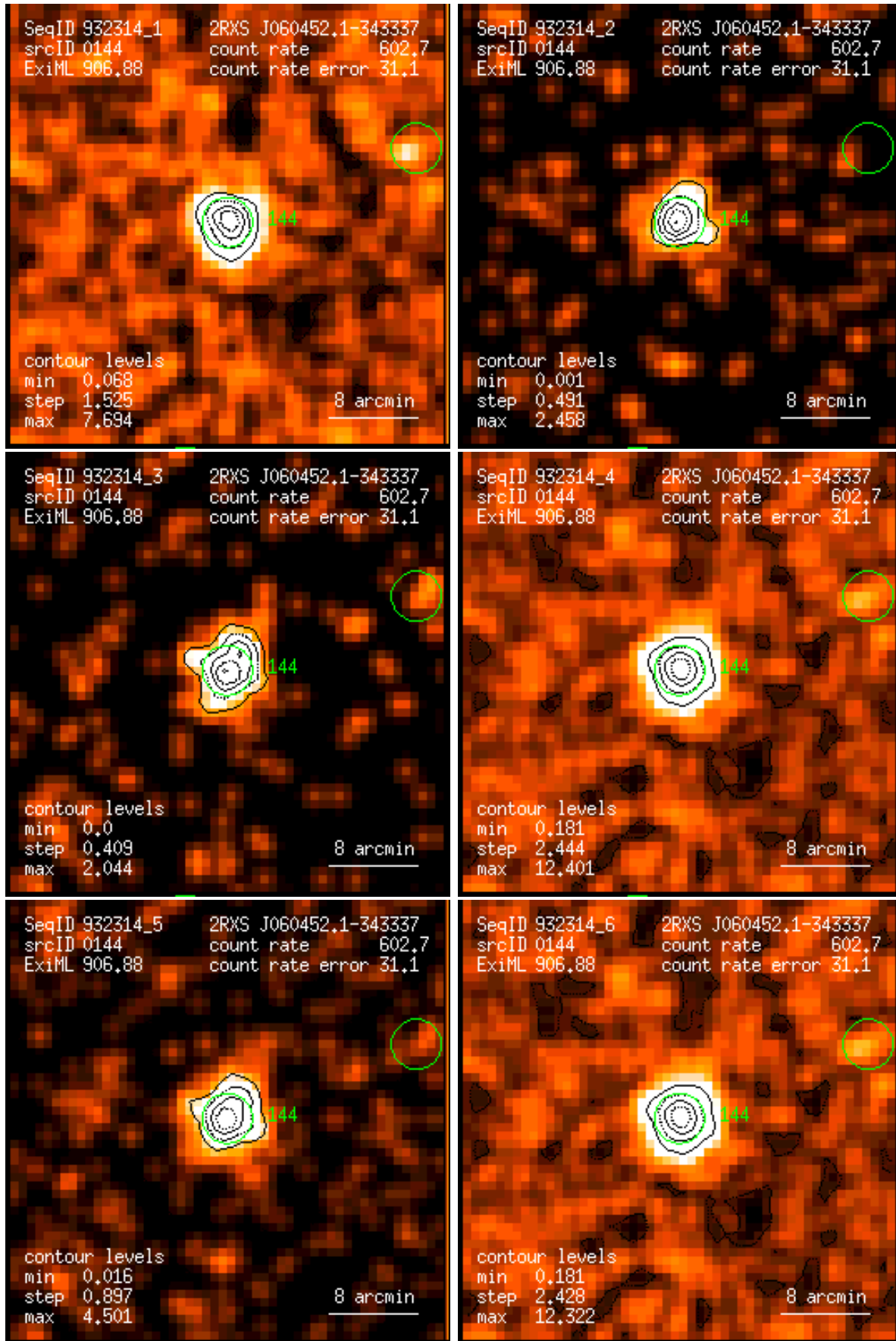
Figure 144: RASS 932314: detection 0144: band rate images, Gaussian filter: (1) PSPC channels 11 – 41, (2) 52 – 90, (3) 91 – 201, (4) 11 – 235, (5) 52 – 201, (6) 11 – 201. Broad band rates in counts/ks. Band rate contour levels in counts/ks/arcmin 2 .
