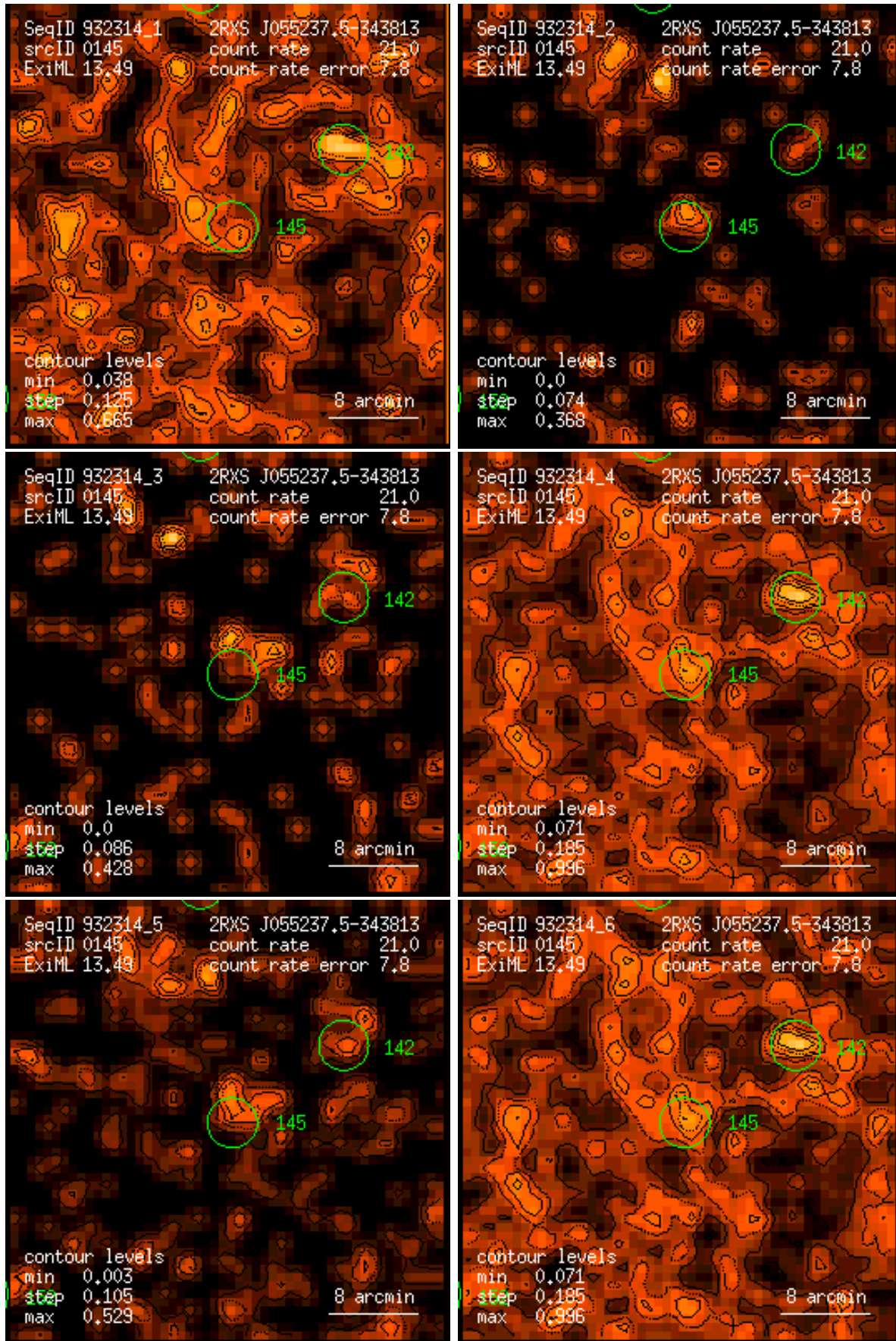
Figure 145: RASS 932314: detection 0145: band rate images, Gaussian filter: (1) PSPC channels 11 – 41, (2) 52 – 90, (3) 91 – 201, (4) 11 – 235, (5) 52 – 201, (6) 11 – 201. Broad band rates in counts/ks. Band rate contour levels in counts/ks/arcmin 2 .
