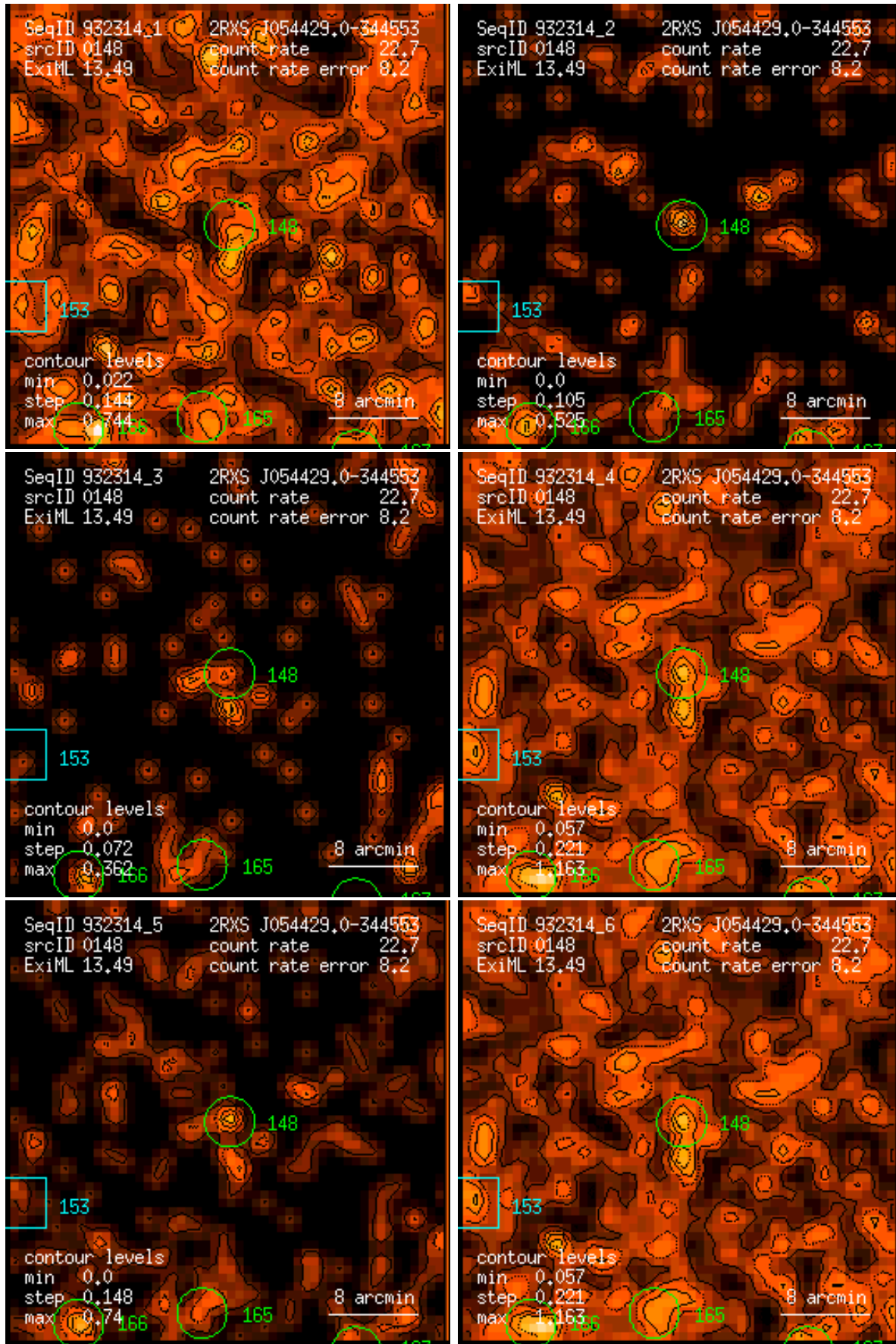
Figure 148: RASS 932314: detection 0148: band rate images, Gaussian filter: (1) PSPC channels 11 – 41, (2) 52 – 90, (3) 91 – 201, (4) 11 – 235, (5) 52 – 201, (6) 11 – 201. Broad band rates in counts/ks. Band rate contour levels in counts/ks/arcmin 2 .
