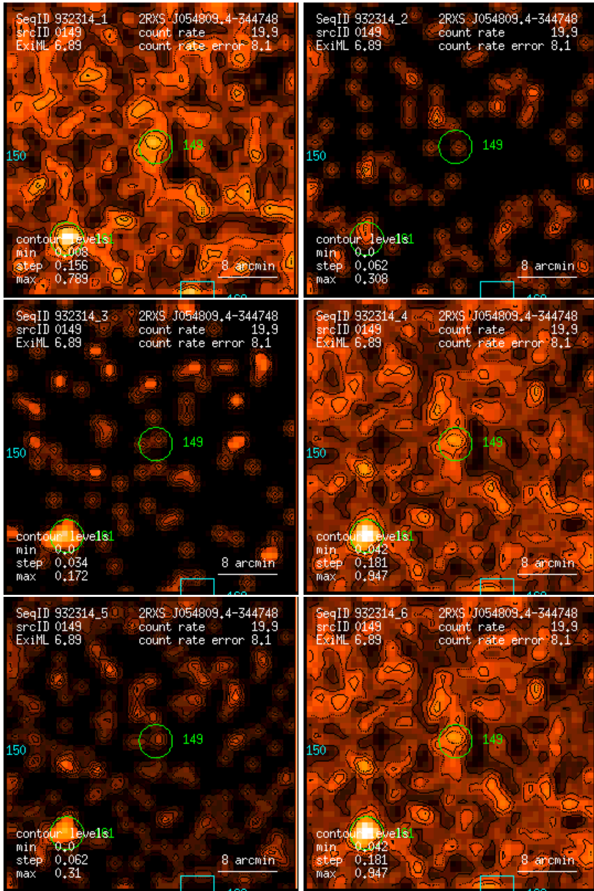
Figure 149: RASS 932314: detection 0149: band rate images, Gaussian filter: (1) PSPC channels 11 – 41, (2) 52 – 90, (3) 91 – 201, (4) 11 – 235, (5) 52 – 201, (6) 11 – 201. Broad band rates in counts/ks. Band rate contour levels in counts/ks/arcmin 2 .
