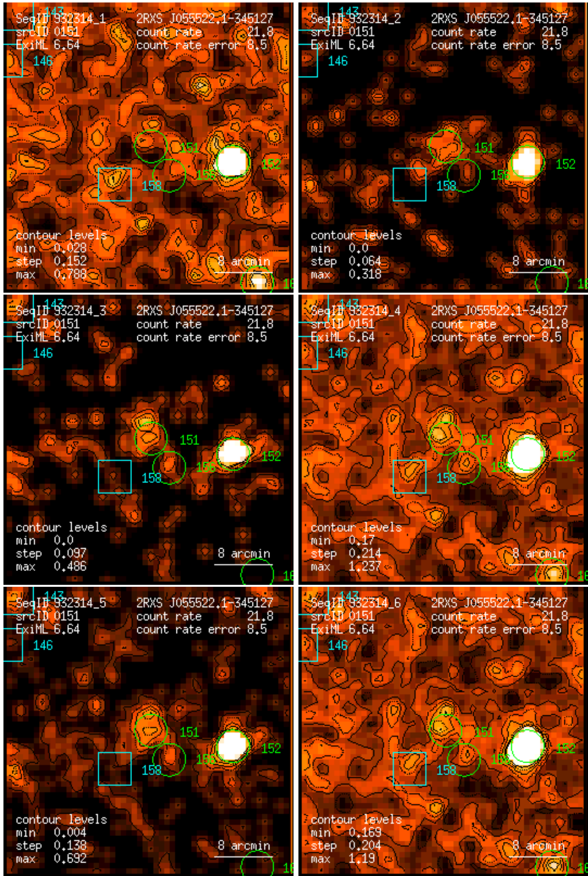
Figure 151: RASS 932314: detection 0151: band rate images, Gaussian filter: (1) PSPC channels 11 – 41, (2) 52 – 90, (3) 91 – 201, (4) 11 – 235, (5) 52 – 201, (6) 11 – 201. Broad band rates in counts/ks. Band rate contour levels in counts/ks/arcmin 2 .
